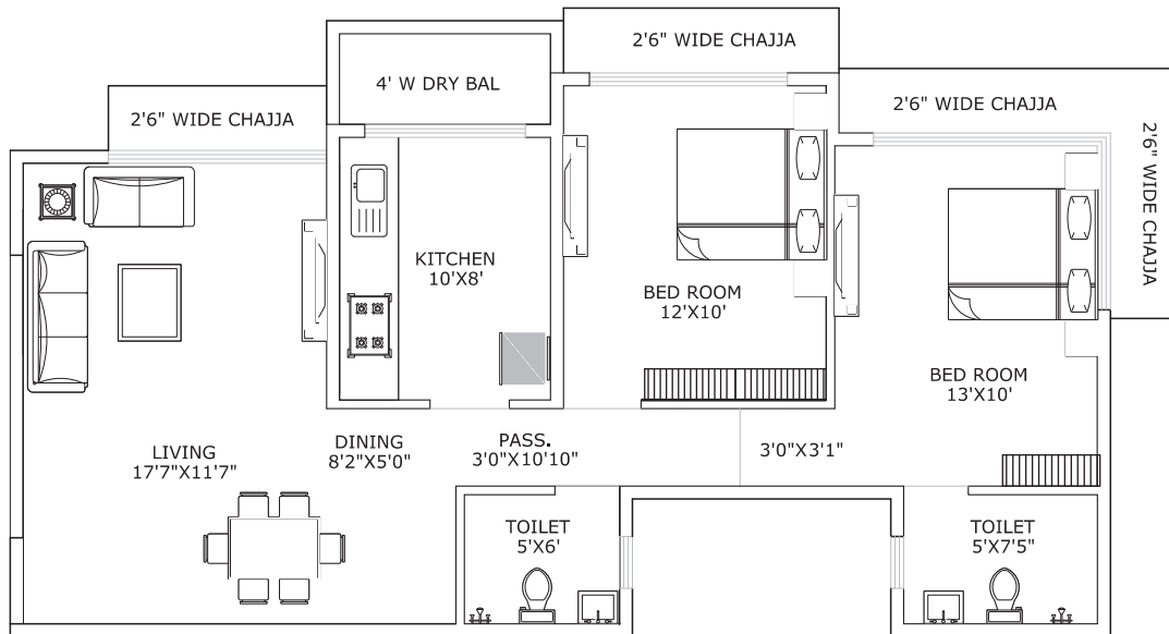
TYPICAL UNIT PLAN - 2 BHK
