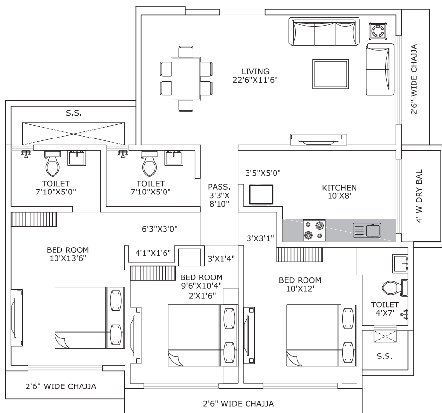
TYPICAL UNIT PLAN - 3 BHK
