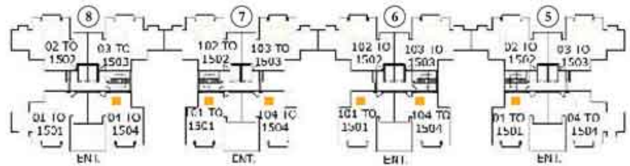
KEY PLAN
