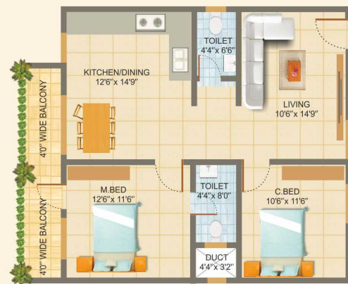
TYPE-10 1097 Sft. FACING East
