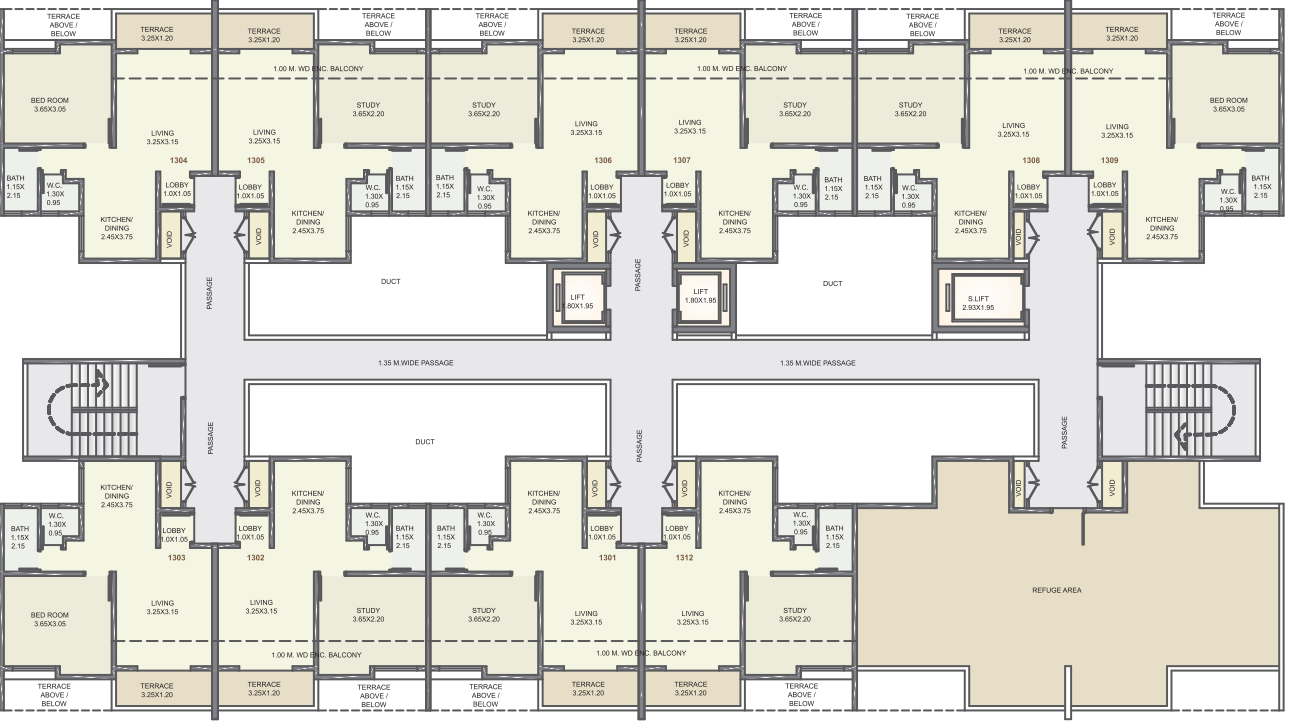
O Building Refuge Floor Plan 13th Floor Plan
