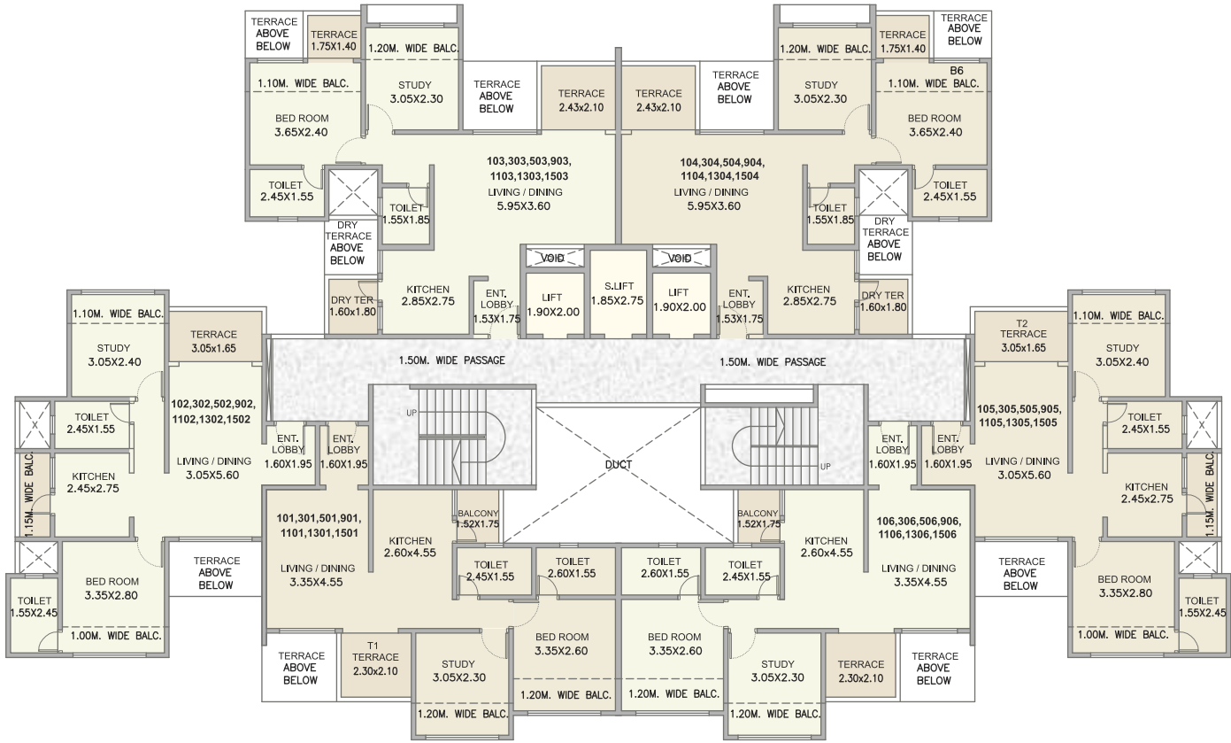
J Building Odd Floor Plan 1st, 3rd, 5th, 9th, 11th, 13th, 15th Floor Plan
