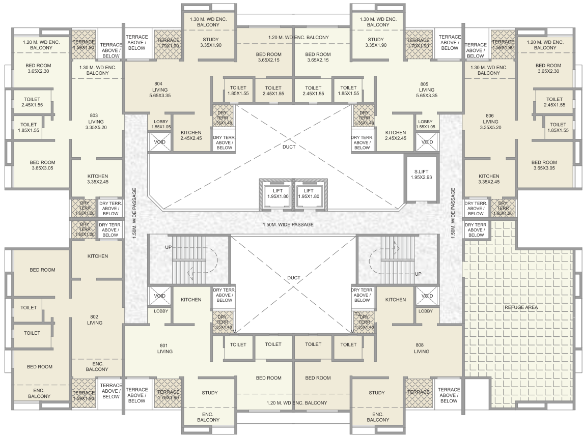
N Building Refuge Floor Plan 8th Floor Plan
