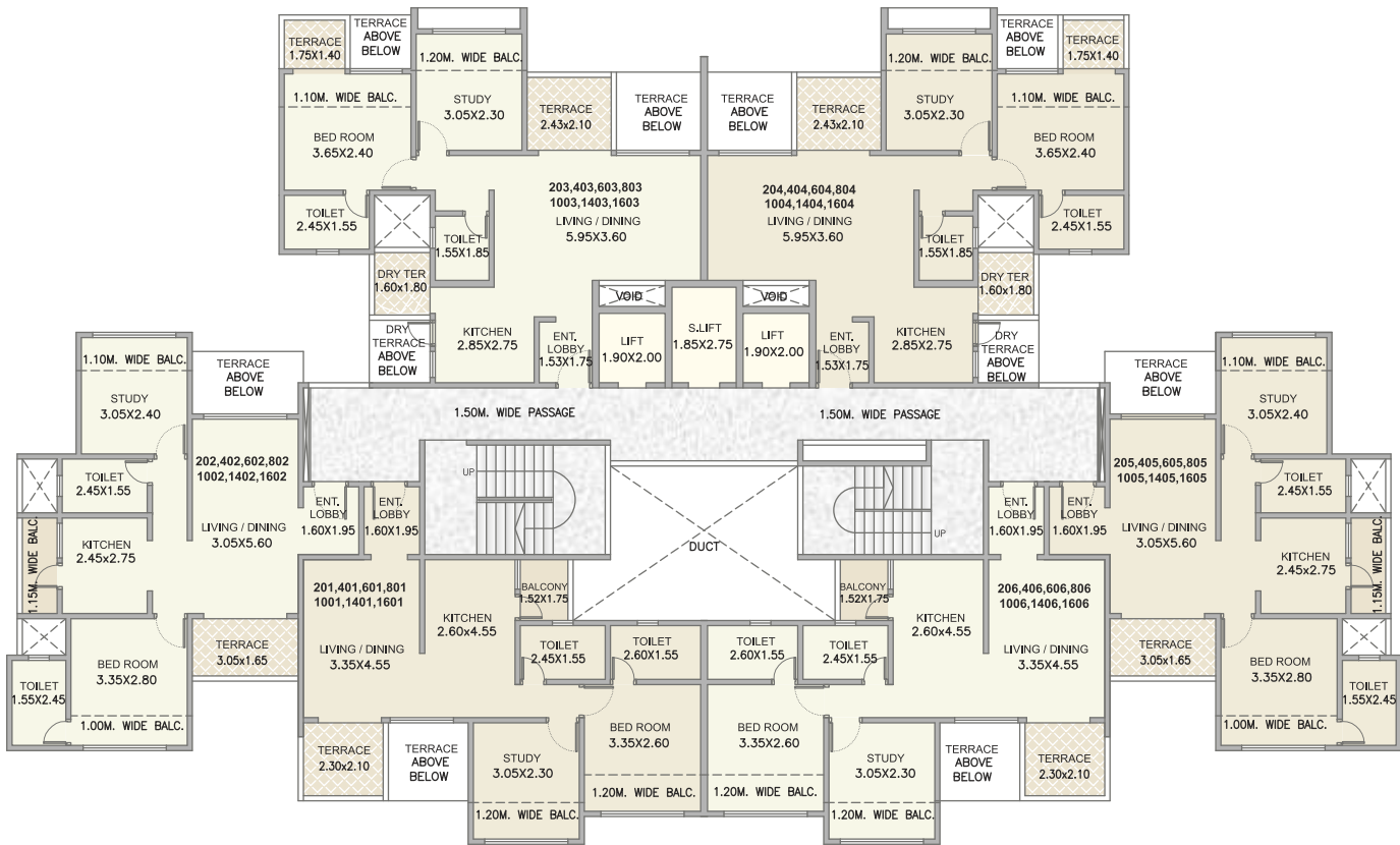
J Building Even Floor Plan 2nd, 4th, 6th, 8th, 10th, 14th, 16th Floor Plan
