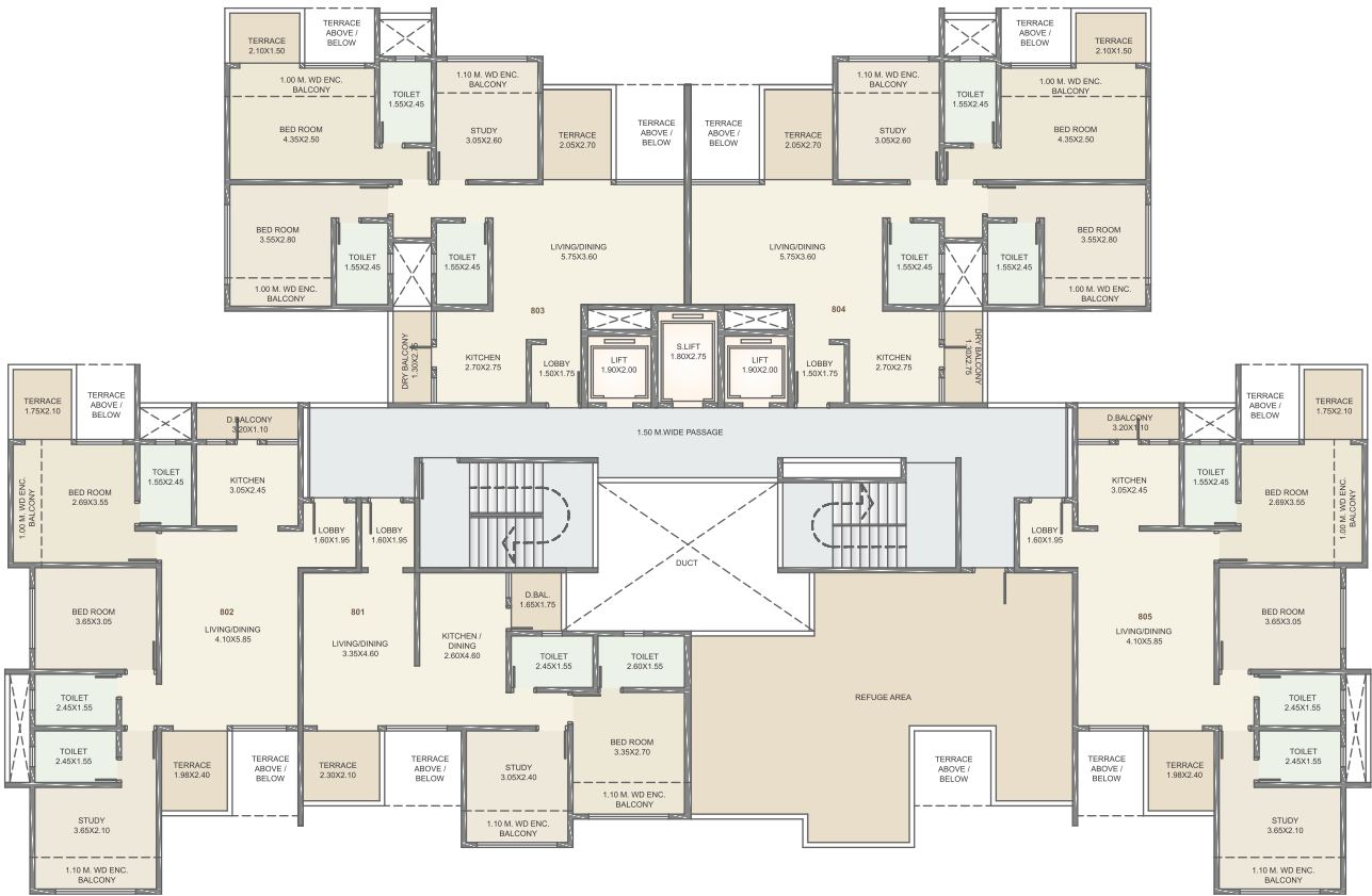
M Building Refuge Floor Plan 8th Floor Plan
