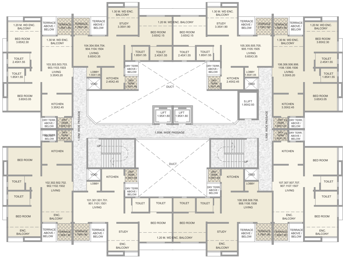
N Building Odd Floor Plan 1st, 3rd, 5th, 7th, 9th, 11th, 15th Floor Plan
