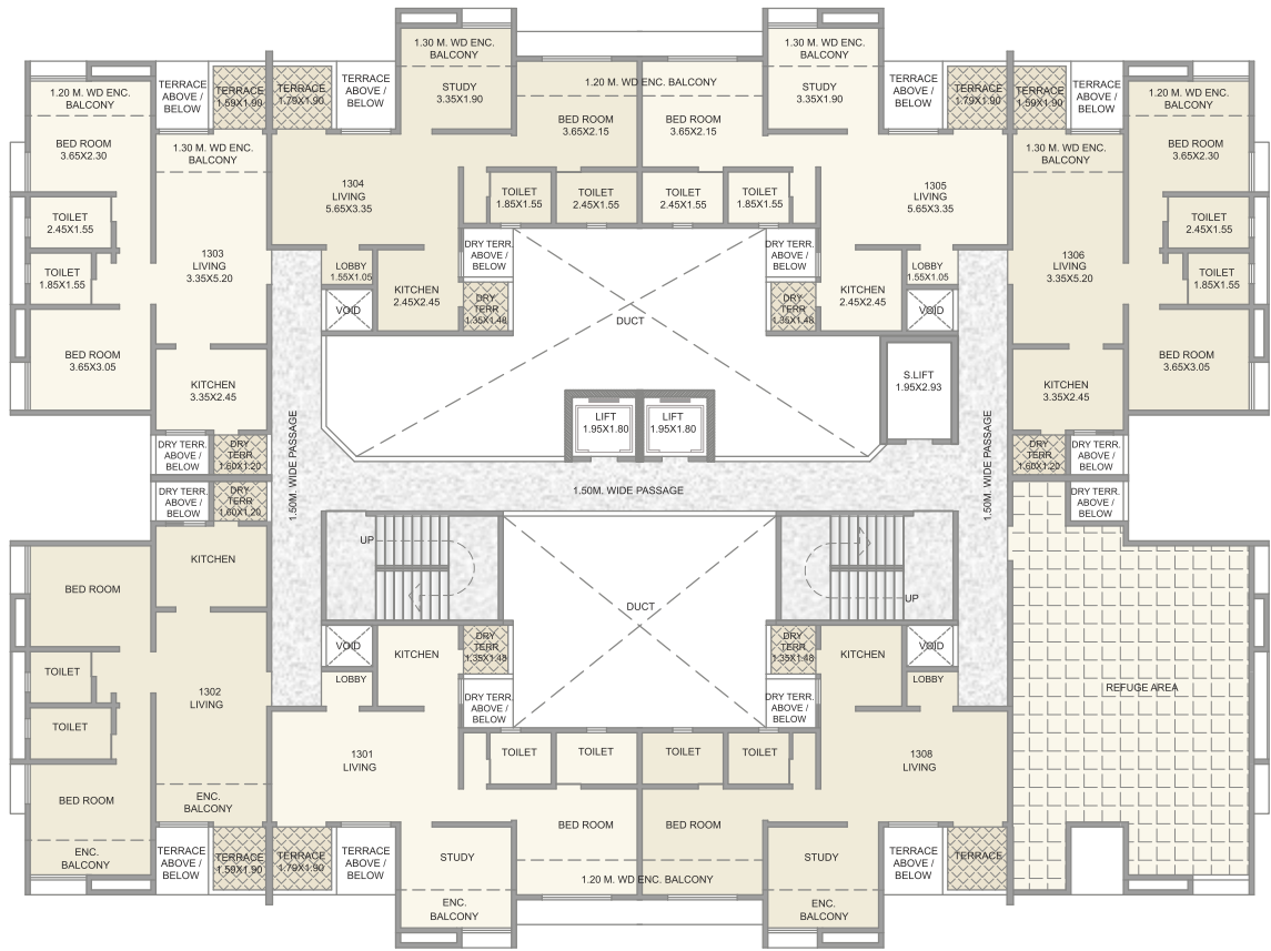
N Building Refuge Floor Plan 13th Floor Plan
