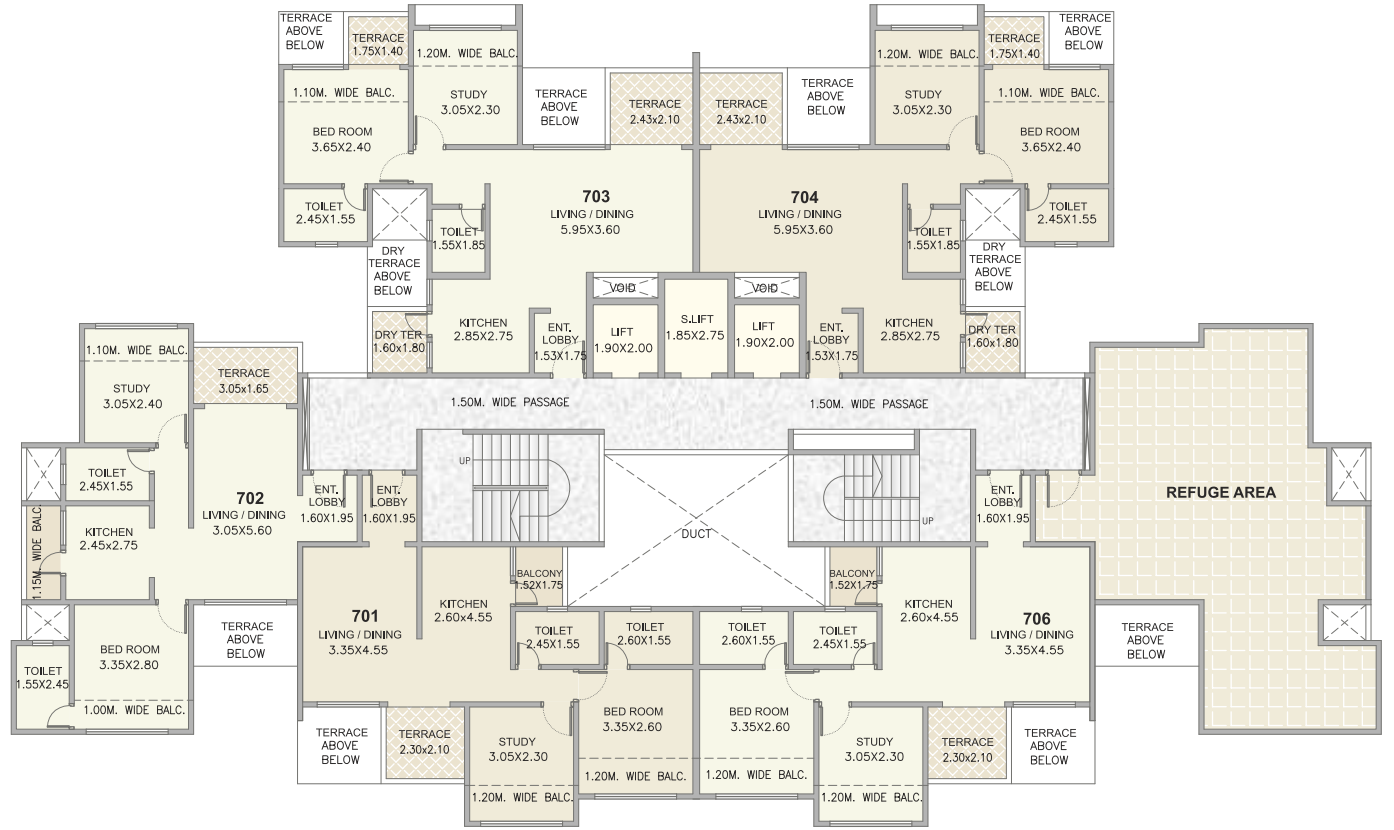
J Building Refuge Floor Plan 7th Floor Plan
