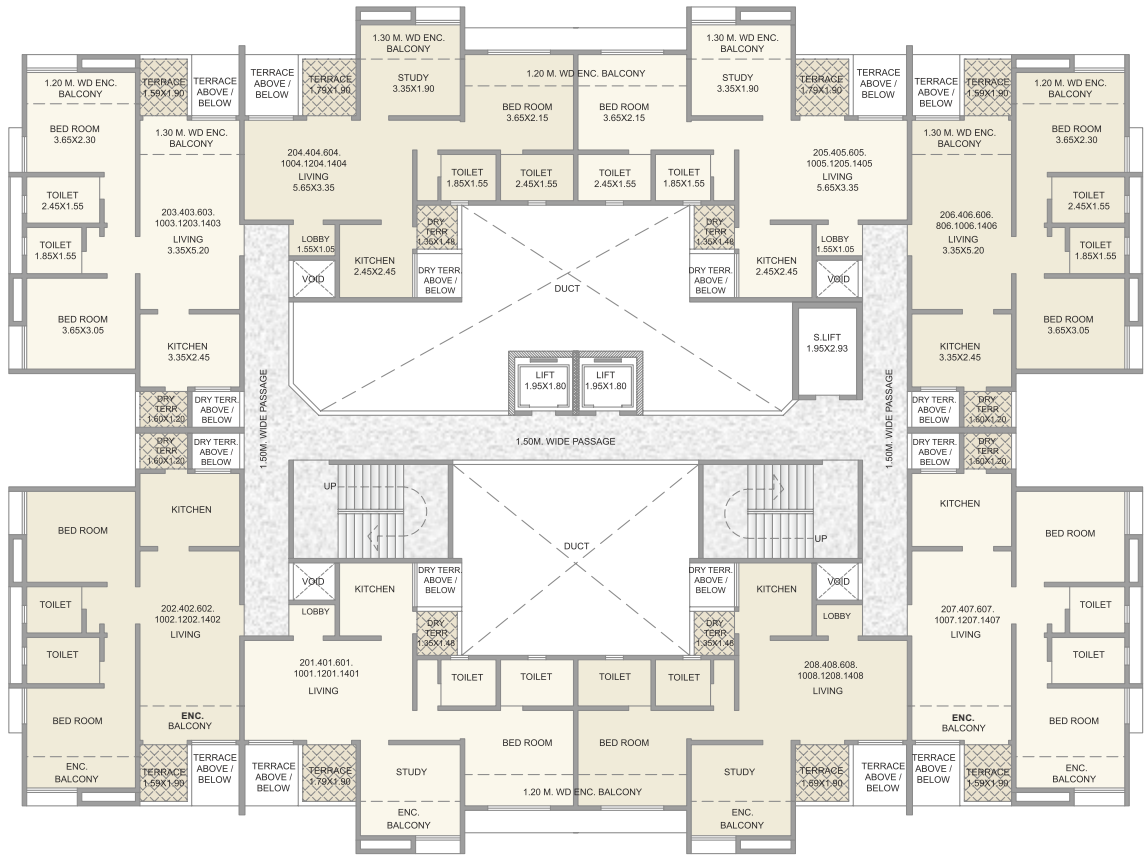
N Building Even Floor Plan 2nd, 4th, 6th, 10th, 12th, 14th Floor Plan
