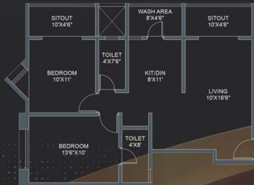
Typical 1st, 2nd, 3rd, 4th, 5th, 6th, 7th Floor Plan
