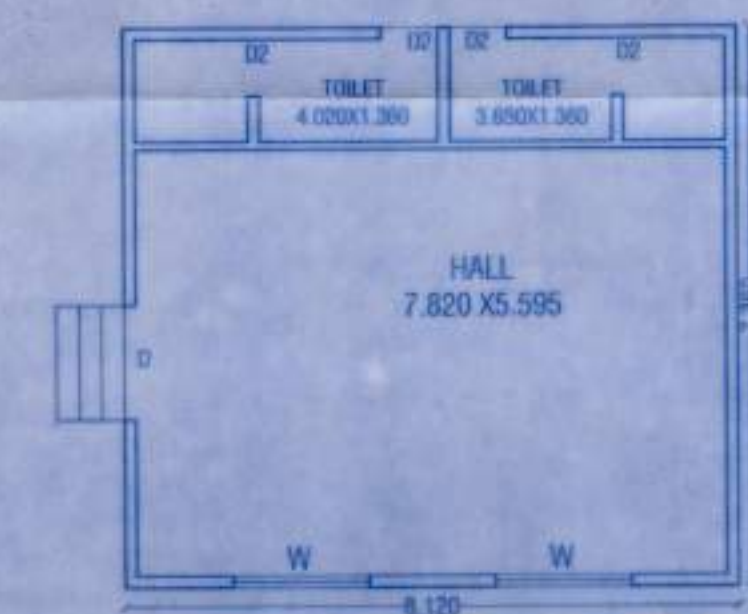
GROUND FLOOR PLAN FOR WING D.
