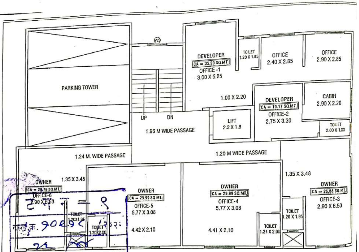
OFFICE FLOOR PLAN - FIRST FLOOR
