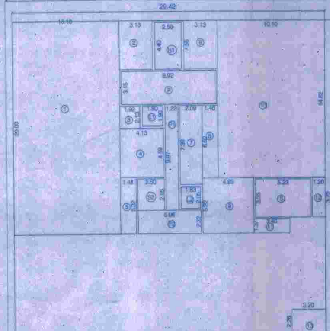
AREA KEY PLAN FOR GROUND FLOOR SCALE: 1:200 (COMM. AREA)
