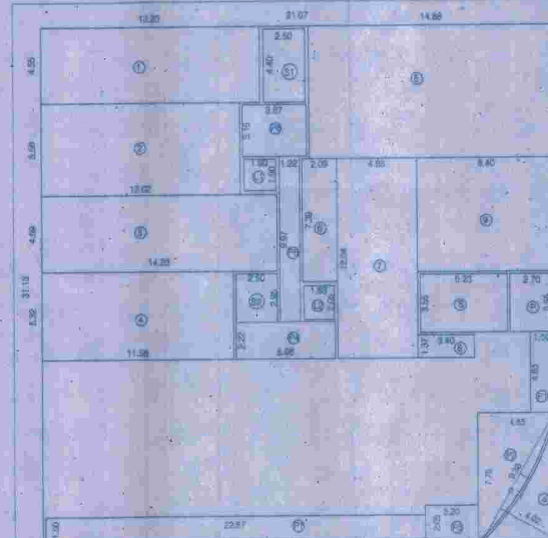
AREA KEY PLAN FOR FIRST FLOOR SCALE: 1:200 (COMM. AREA)
