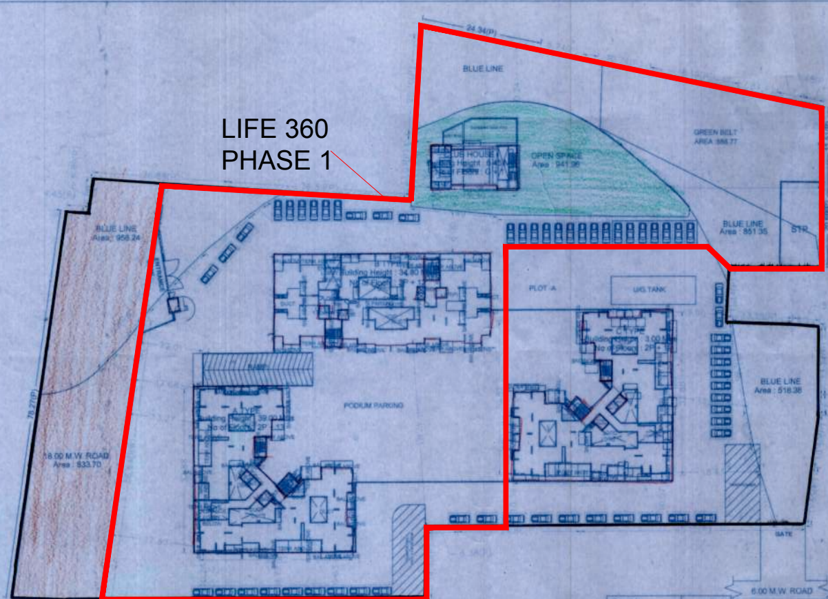
LAYOUT PLAN (Scale - 1:500)
