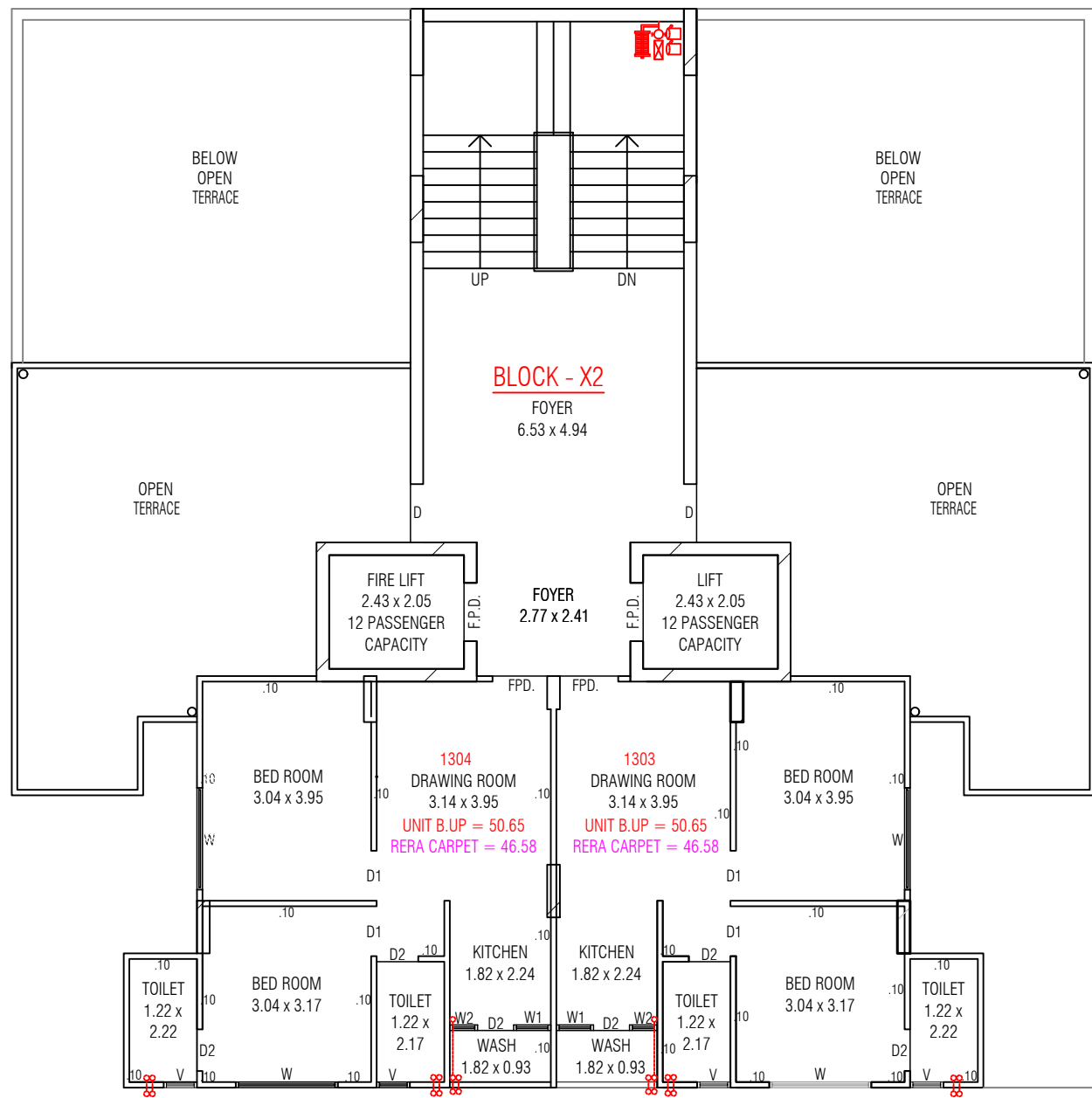
13.TH FLOOR PLAN X1 + X2
