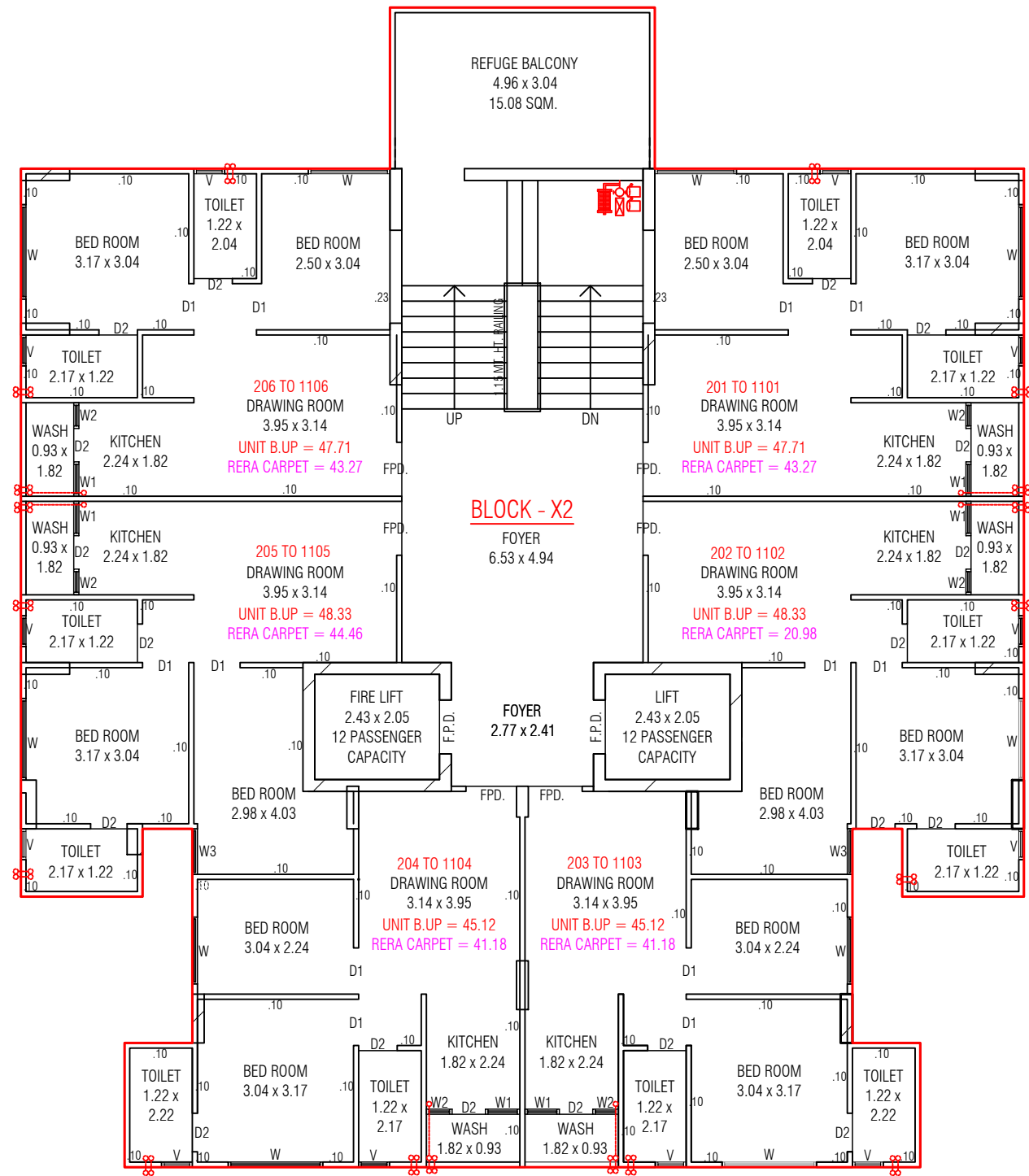
5.TH, 8TH FLOOR PLAN (REFUGE FLOOR) X1 + X2
