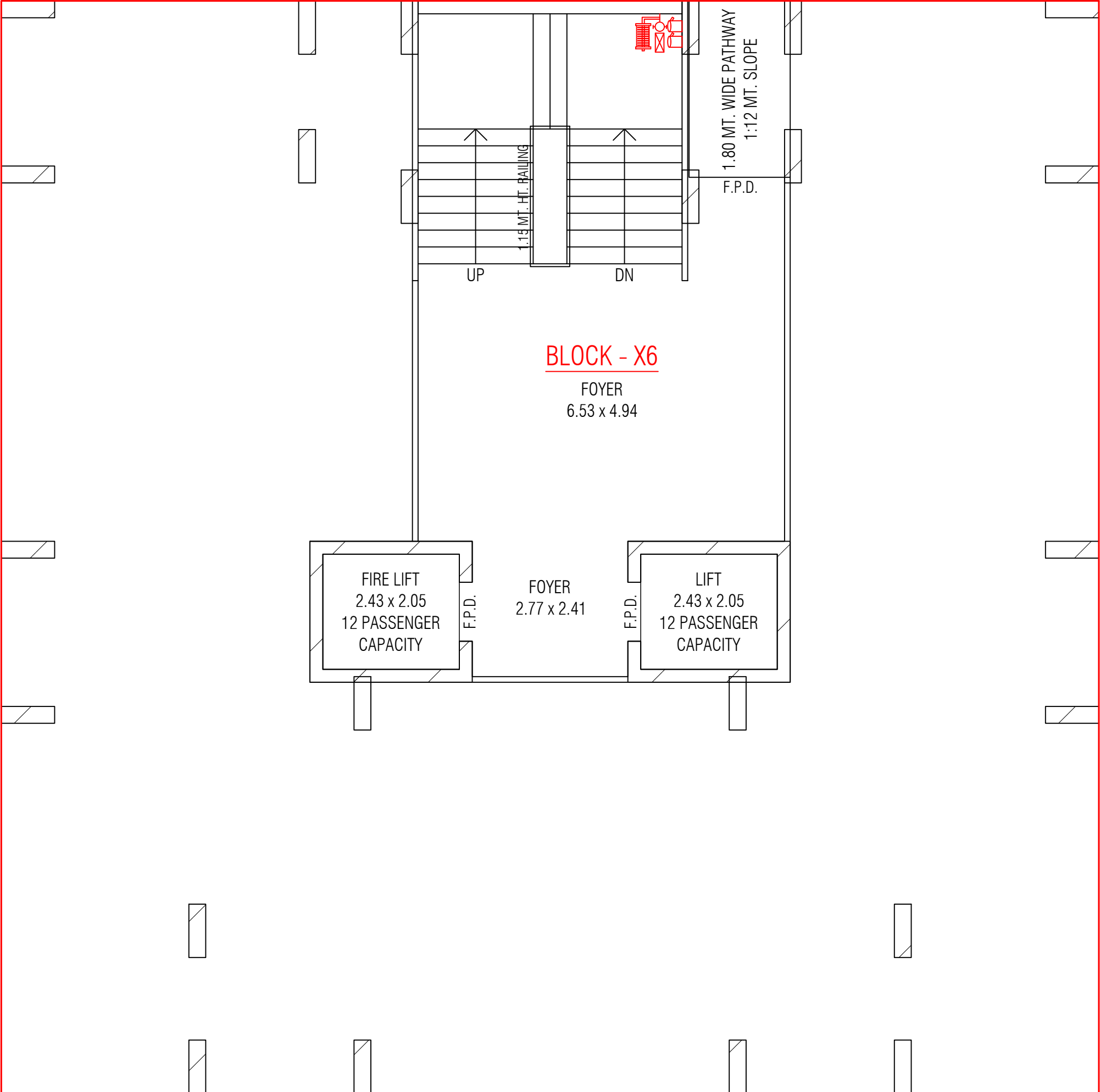
GROUND FLOOR PLAN-X6
