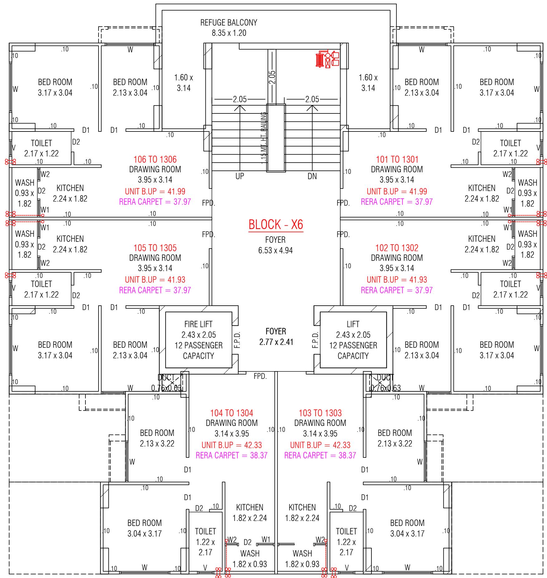
5TH, 8TH & 12TH FLOOR PLAN ( REFUGE AREA PLAN )-X6
