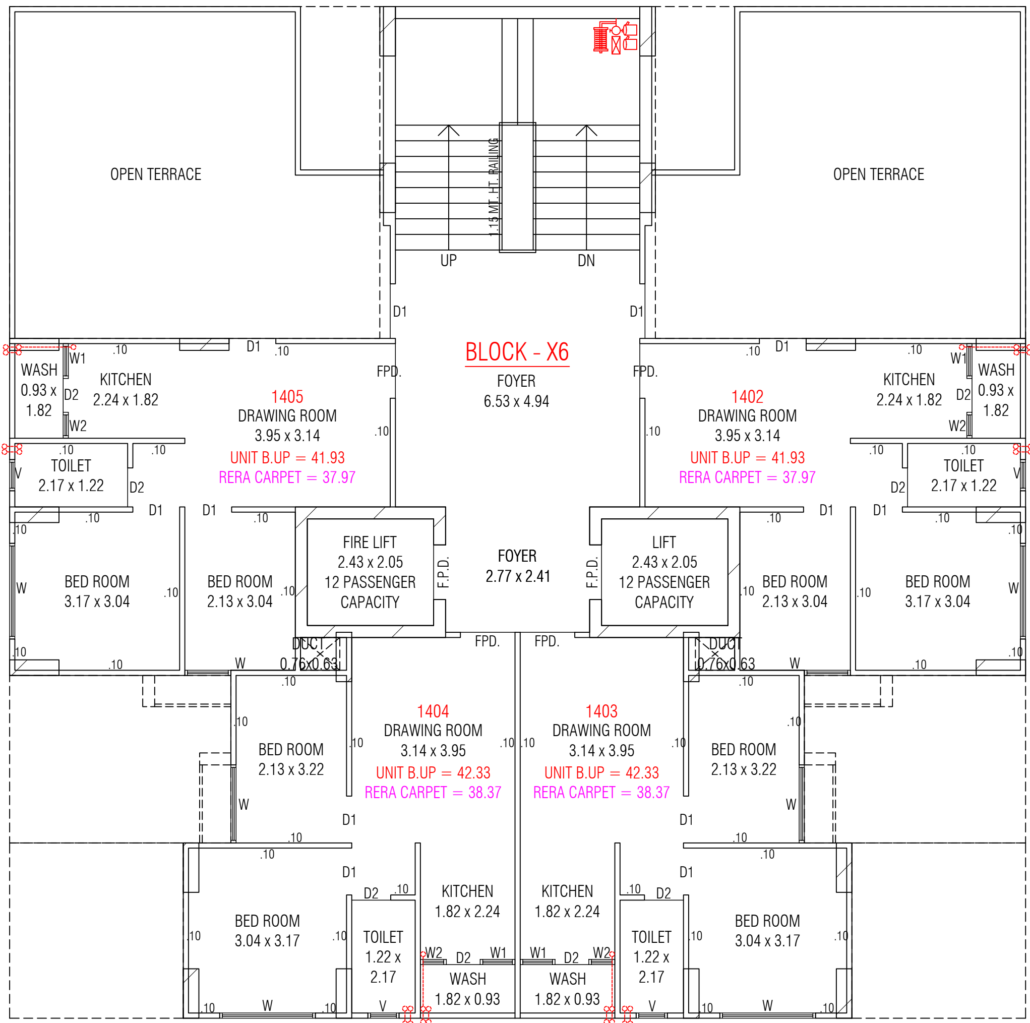
14TH FLOOR PLAN-X6 025
