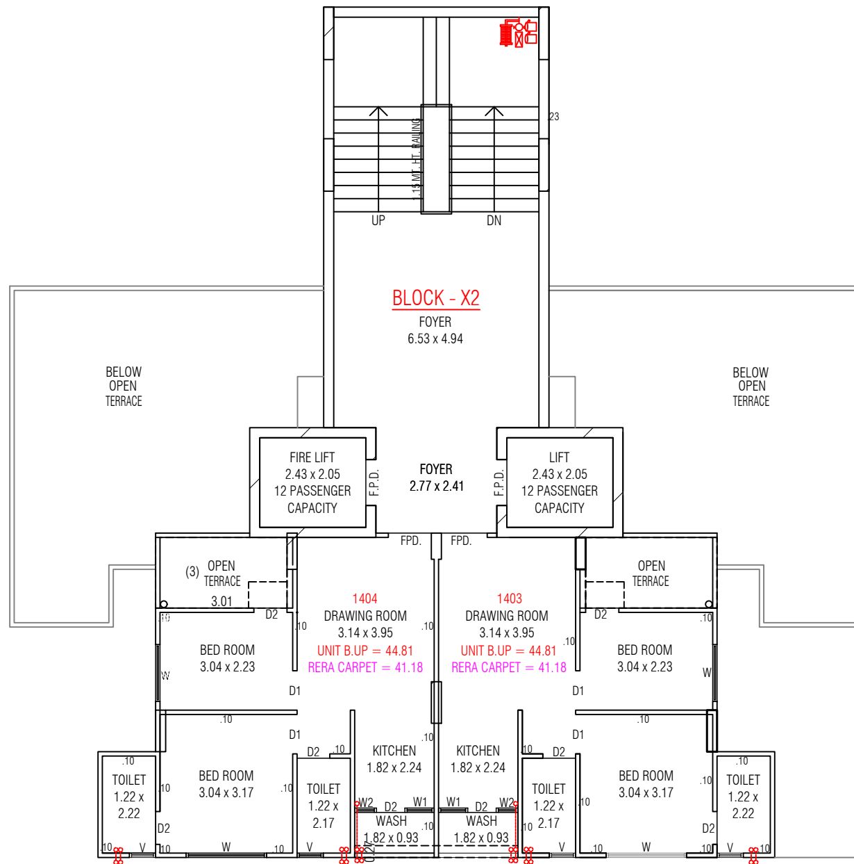
14.TH FLOOR PLAN X1 + X2
