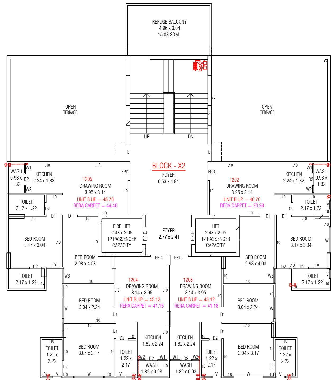
12.TH FLOOR PLAN (REFUGE FLOOR) X1 + X2
