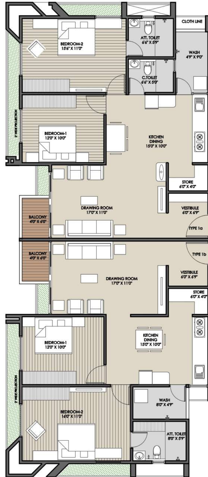
2 BHK UNIT TYPE -A
