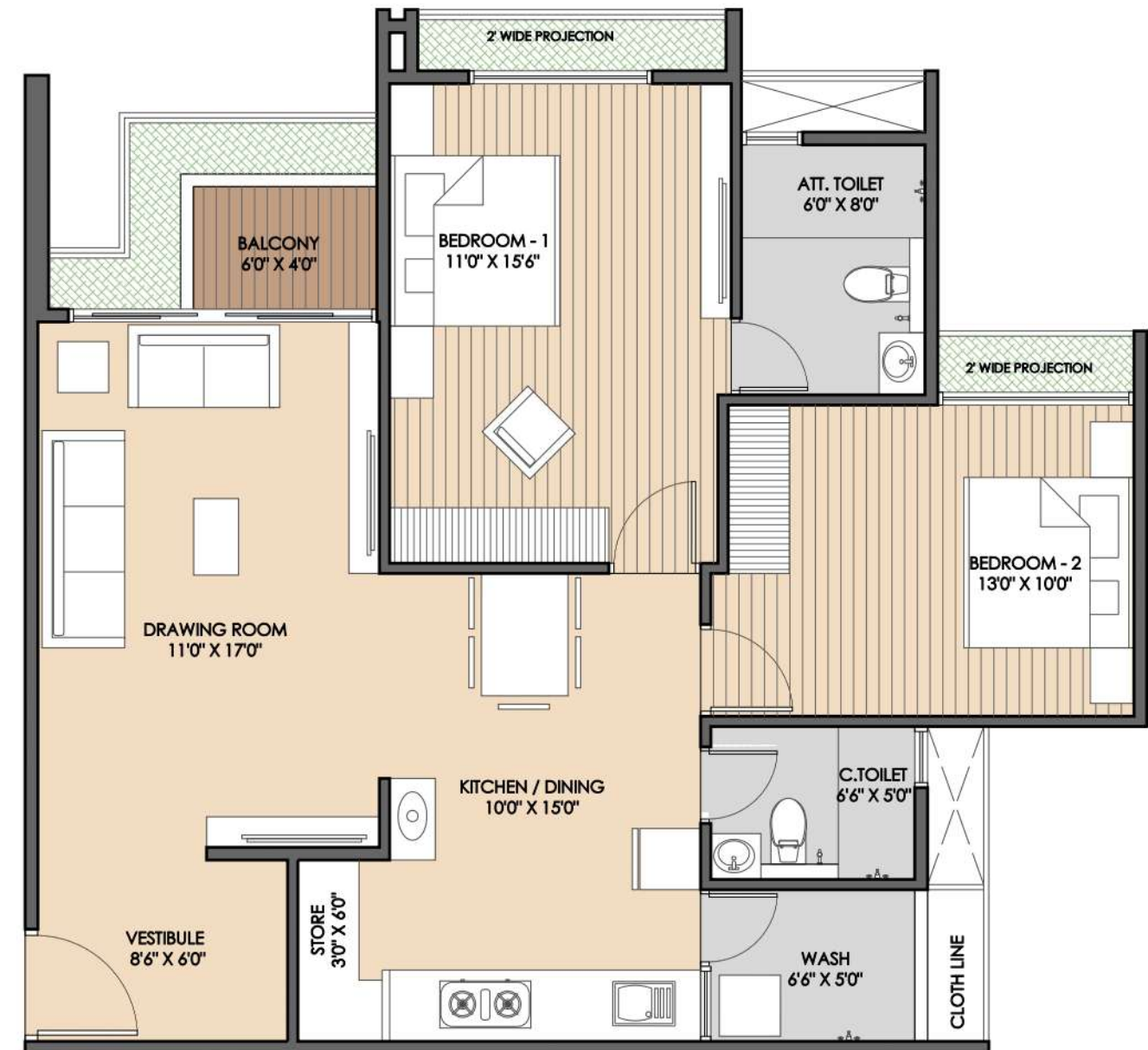
2 BHK UNIT TYPE -B
