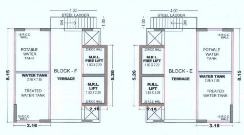
WATER TANK & M.R.L. LIFT
