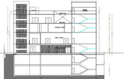
SECTION S1 (SCALE 1:200) (CLUB HOUSE-2)
