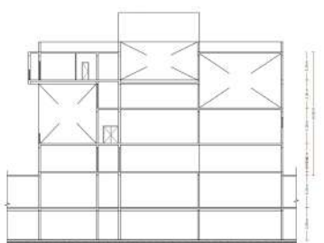
SECTION S2 (SCALE 1:200) (CLUB HOUSE-2)
