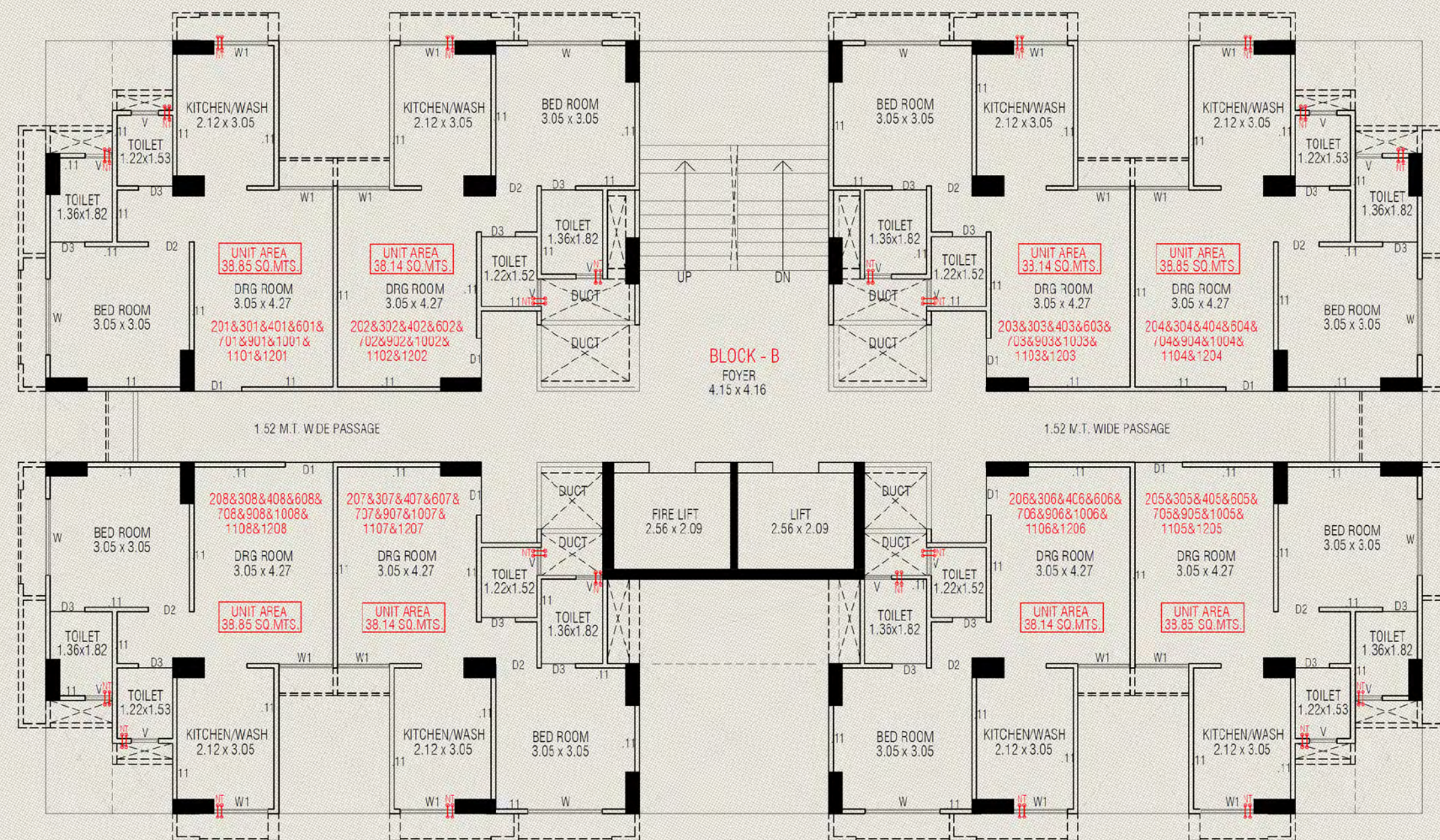
2ND & 3RD & 4TH & 6TH & 7TH & 9TH & 10TH & 11TH & 12TH FLOOR PLAN
