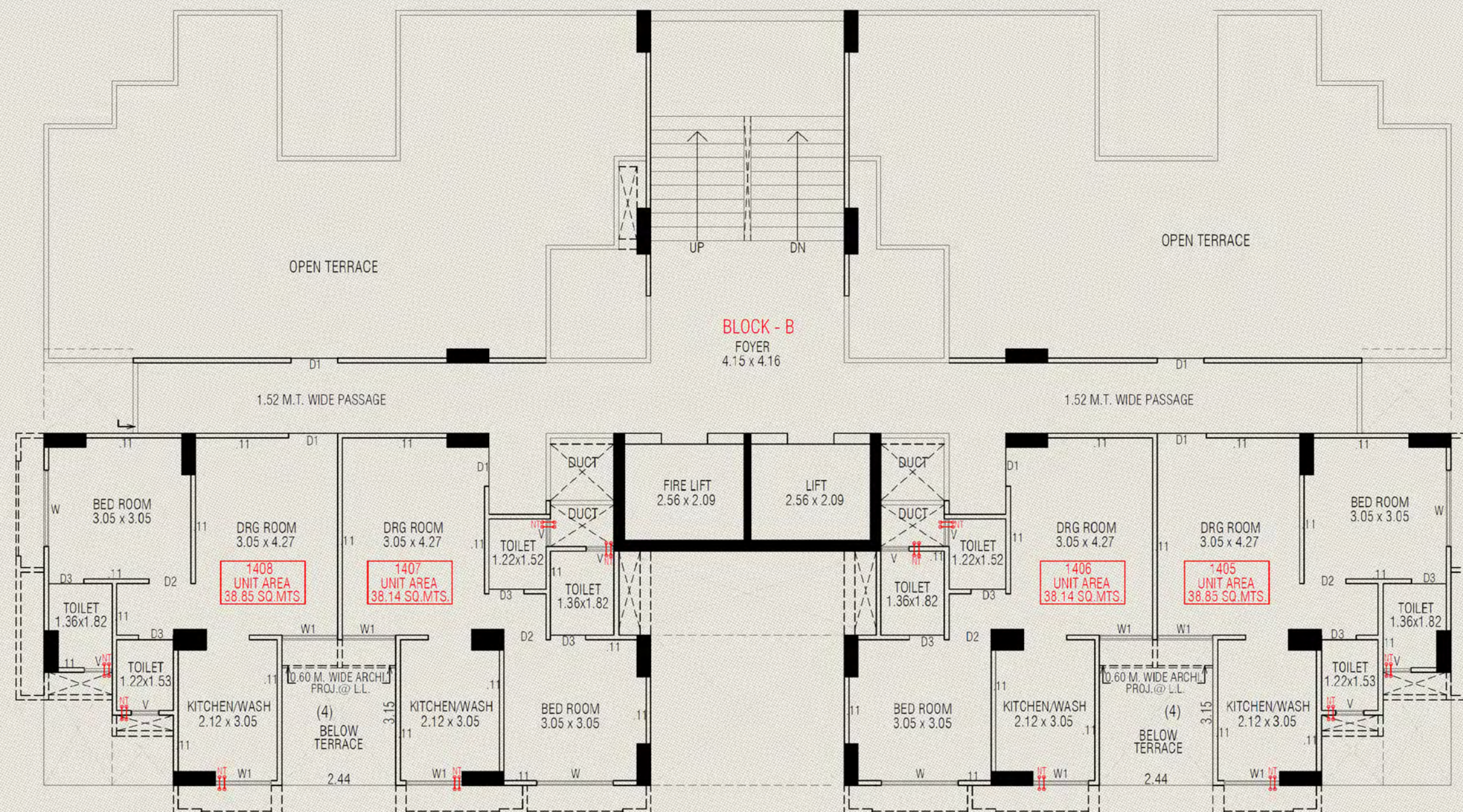
14TH FLOOR PLAN
