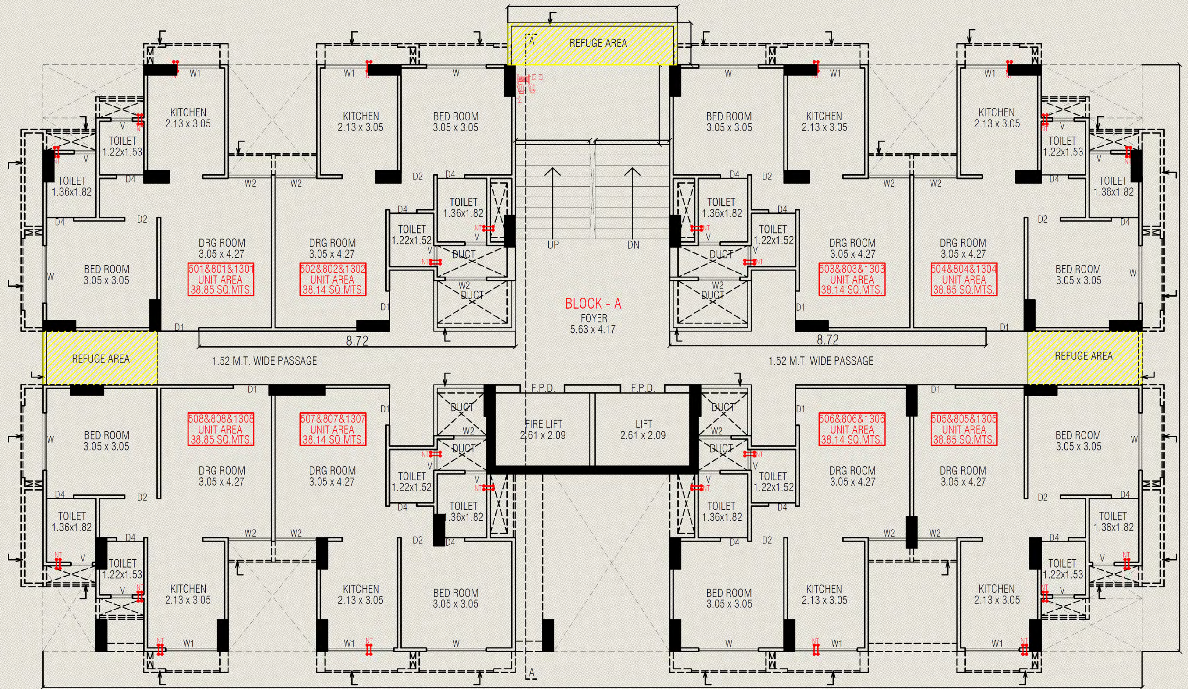
5TH & 8TH & 13TH FLOOR PLAN ( REFUGE AREA)
