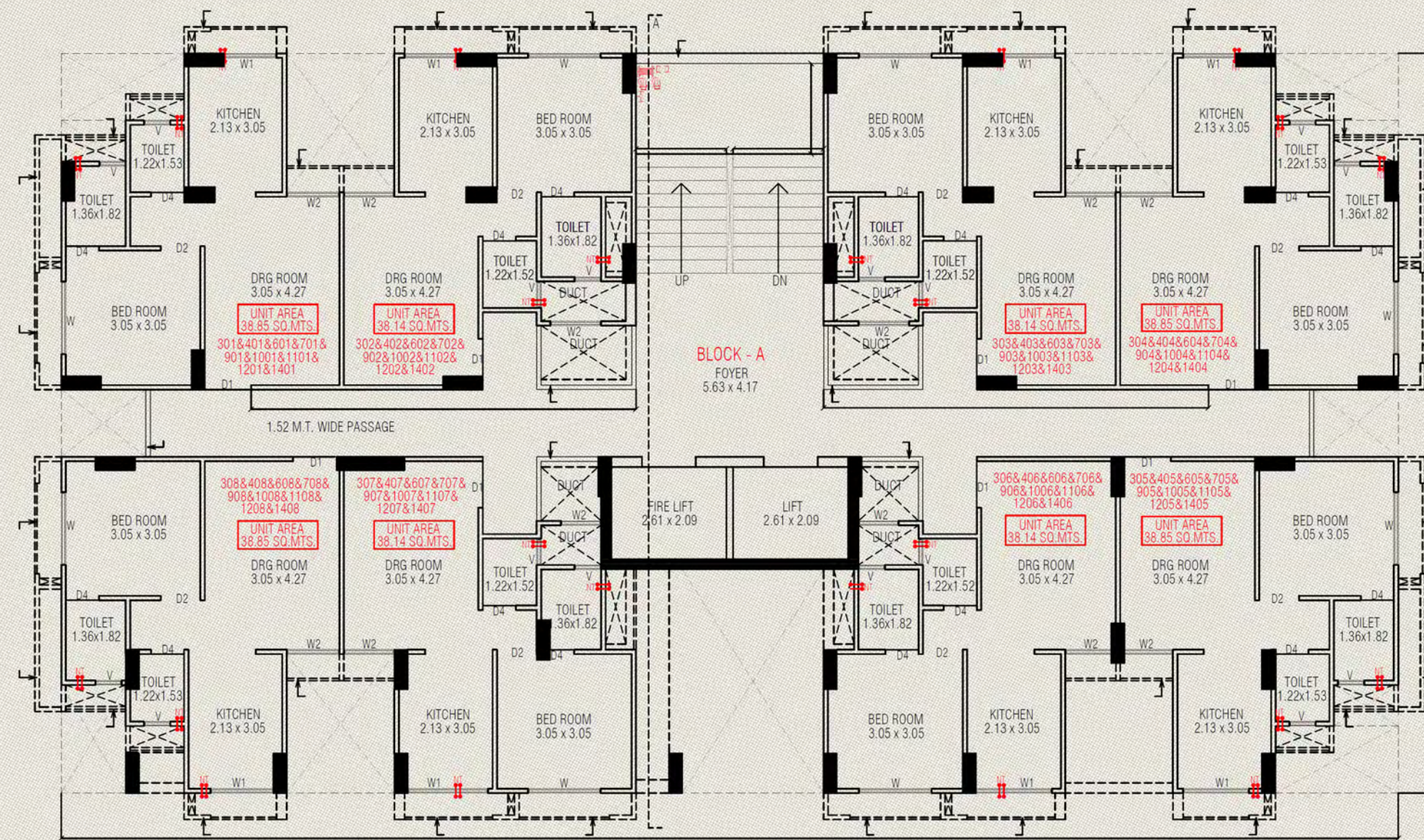
3RD & 4TH & 6TH & 7TH & 9TH & 10TH & 11TH & 12TH & 14TH FLOOR PLAN
