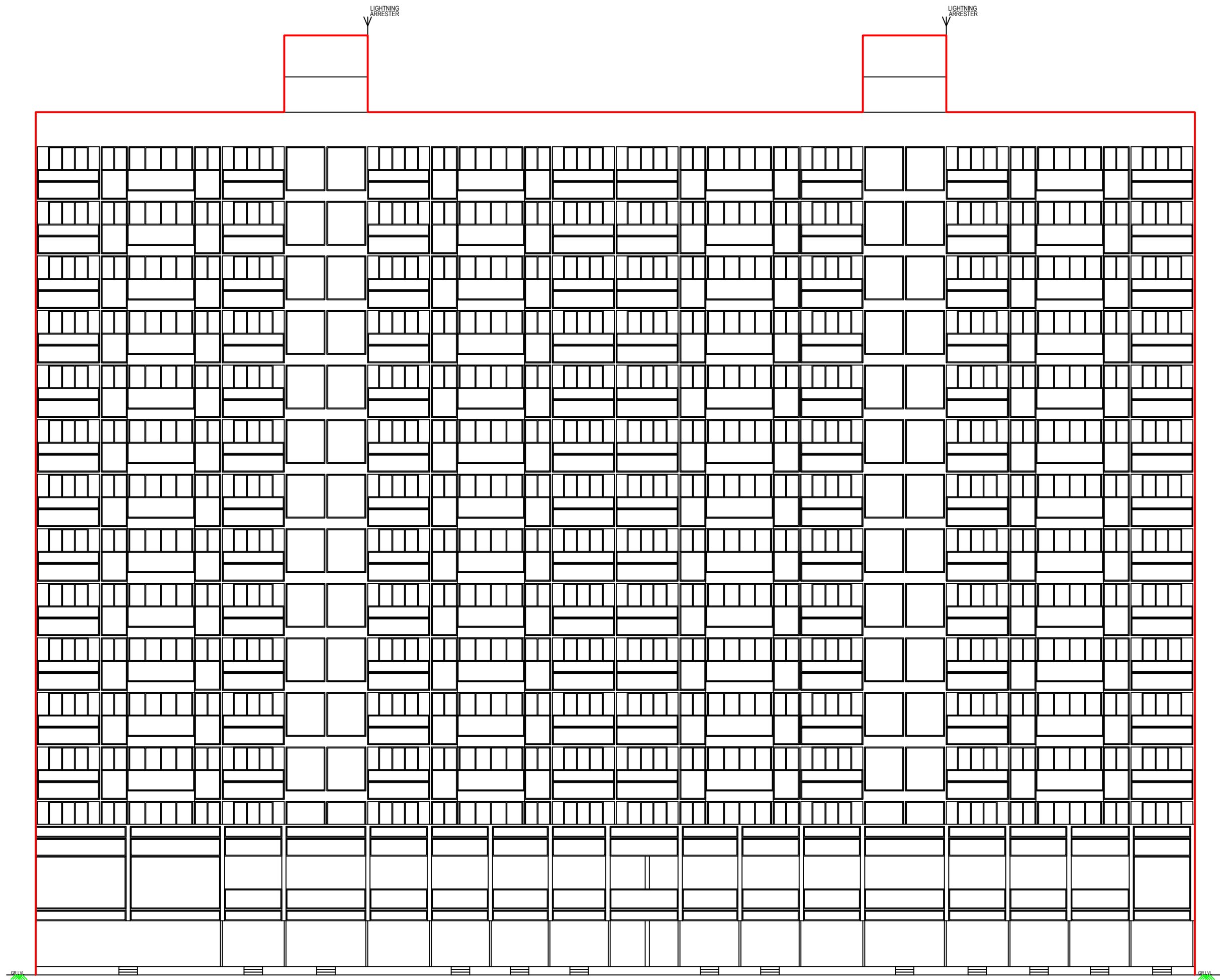
FRONT ELEVATION - 2
