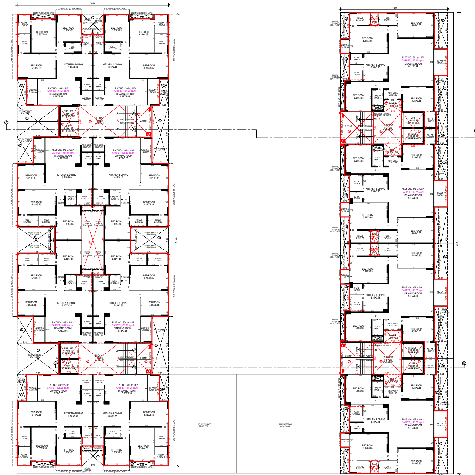
3rd to 14th FLOOR PLAN
