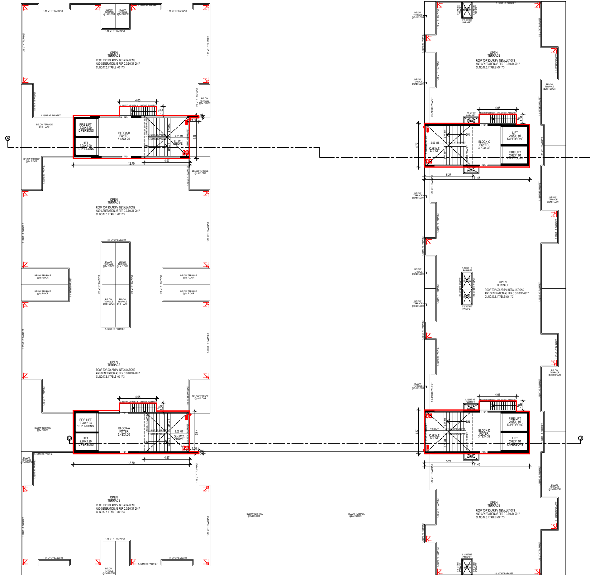
STAIR CABIN & TERRACE PLAN
