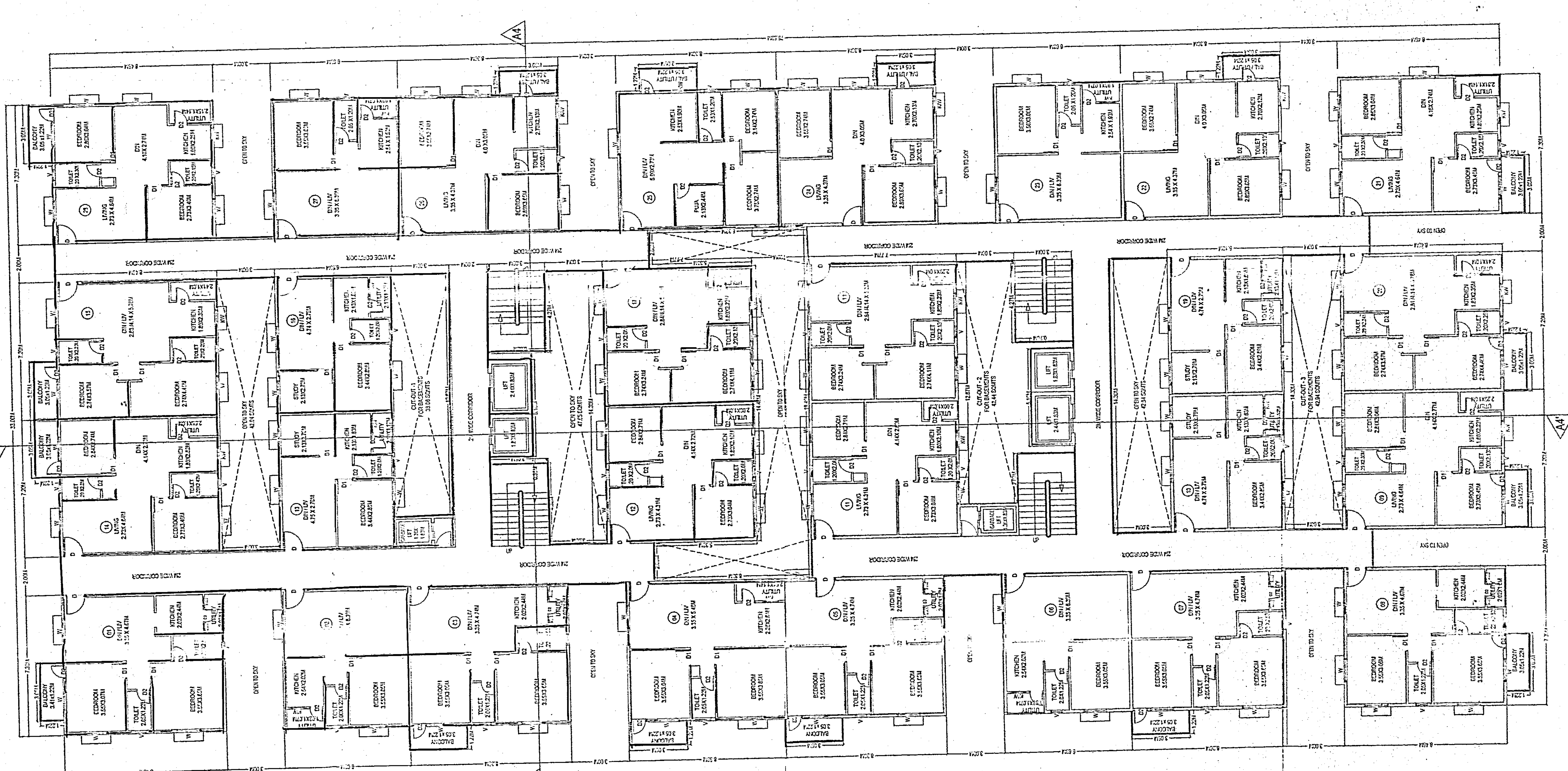
BLOCK-A4 TYPICAL FLOOR PLAN (2nd, 4th, 6th & 8th Floor)
