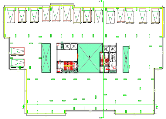
STILT FLOOR PLAN (SCALE 1:100)
