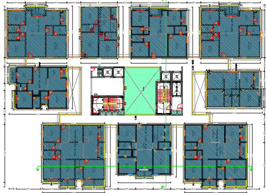
FIRST FLOOR PLAN (Proposed) (SCALE 1:100)
