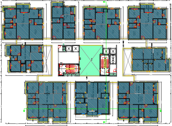
SECOND FLOOR PLAN (Proposed) (SCALE 1:100)
