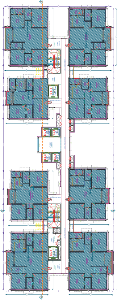
SECOND FLOOR PLAN (Proposed) (SCALE 1:100)
