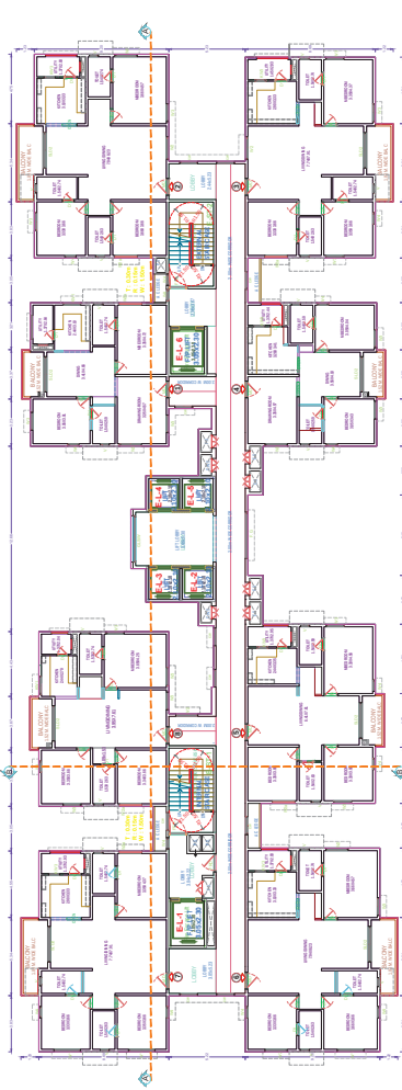
TYPICAL - 4 - 7, 12 - 14, 19, 21 - 26 FLOOR PLAN (Proposed) (SCALE 1:100)
