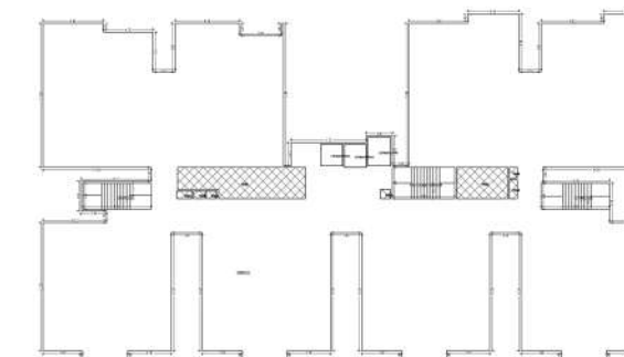
TERRACE FLOOR PLAN (SCALE 1:200) (TOWER NO 2)
