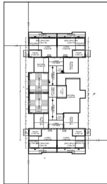
SEVENTH FLOOR PLAN
