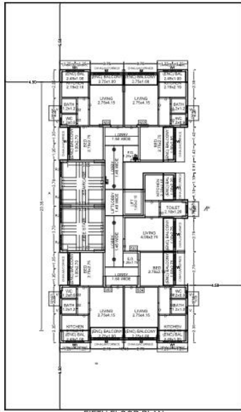
FIFTH FLOOR PLAN
