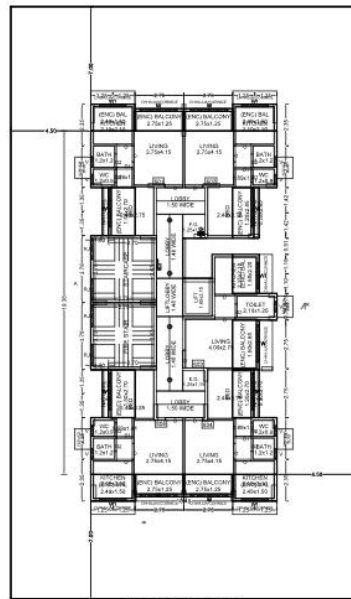
SIXTH FLOOR PLAN
