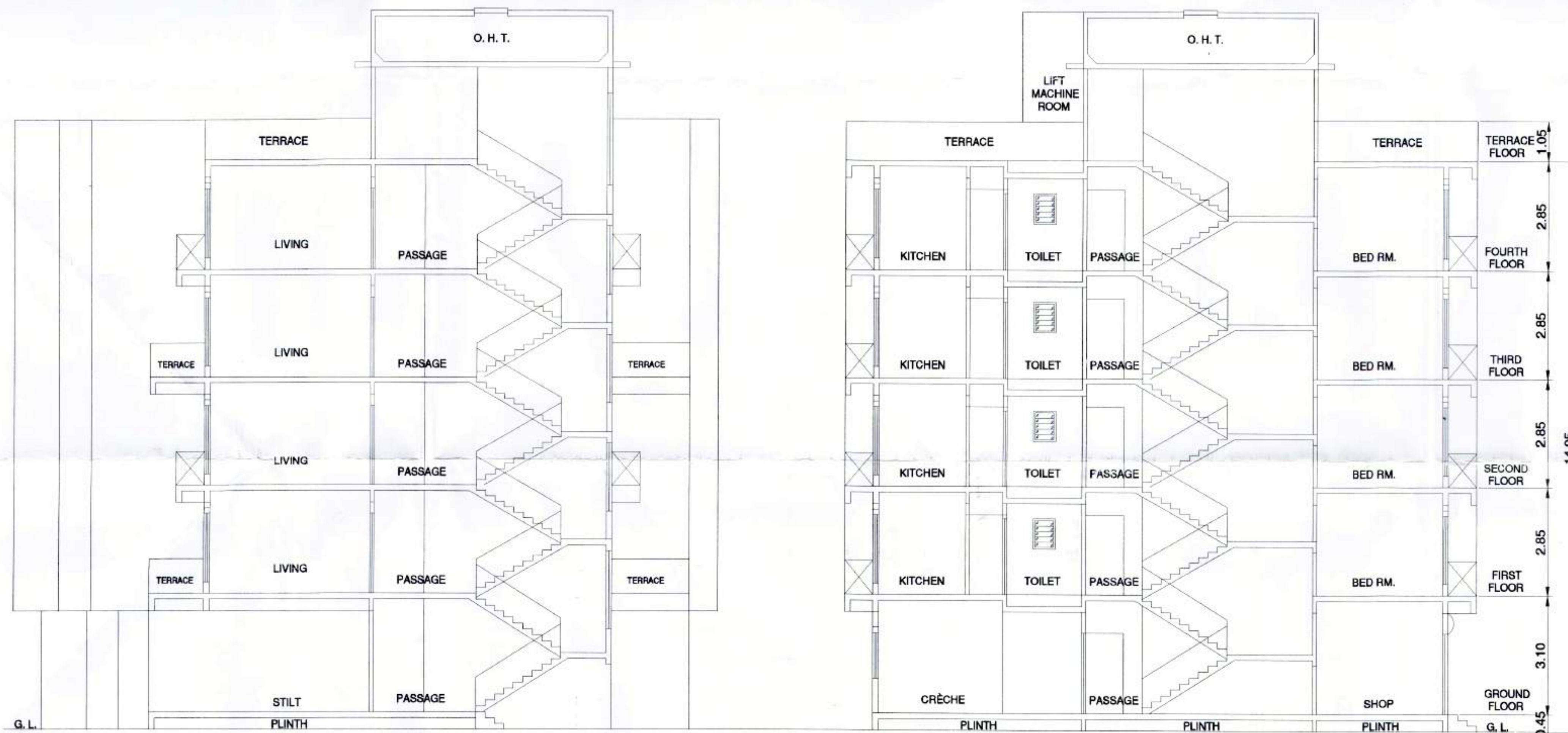
SECTION = A - A' (SCALE = 1 : 100), WING - A & B.
