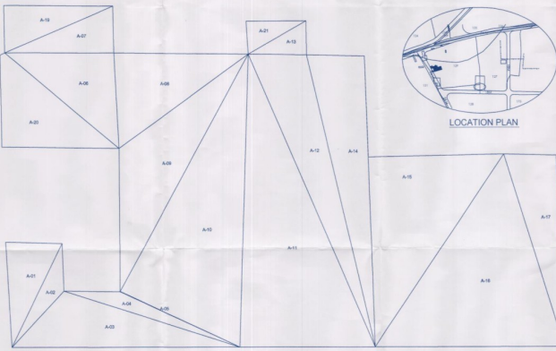
Triangulation (Scale - 1:500)
