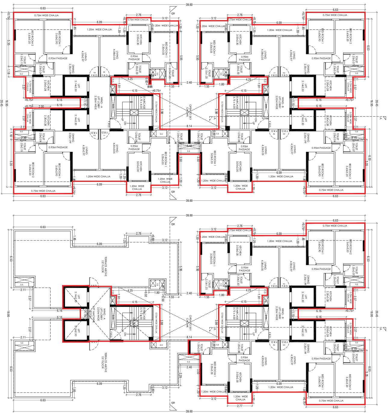
TYPICAL FLOOR PLAN (2ND-6TH, 8TH-10TH) SCALE = 1:100
