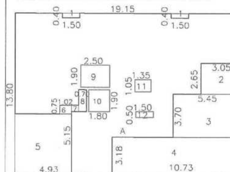
BUILT-UP AREA STATEMENT : FIRST FLOOR AREA
