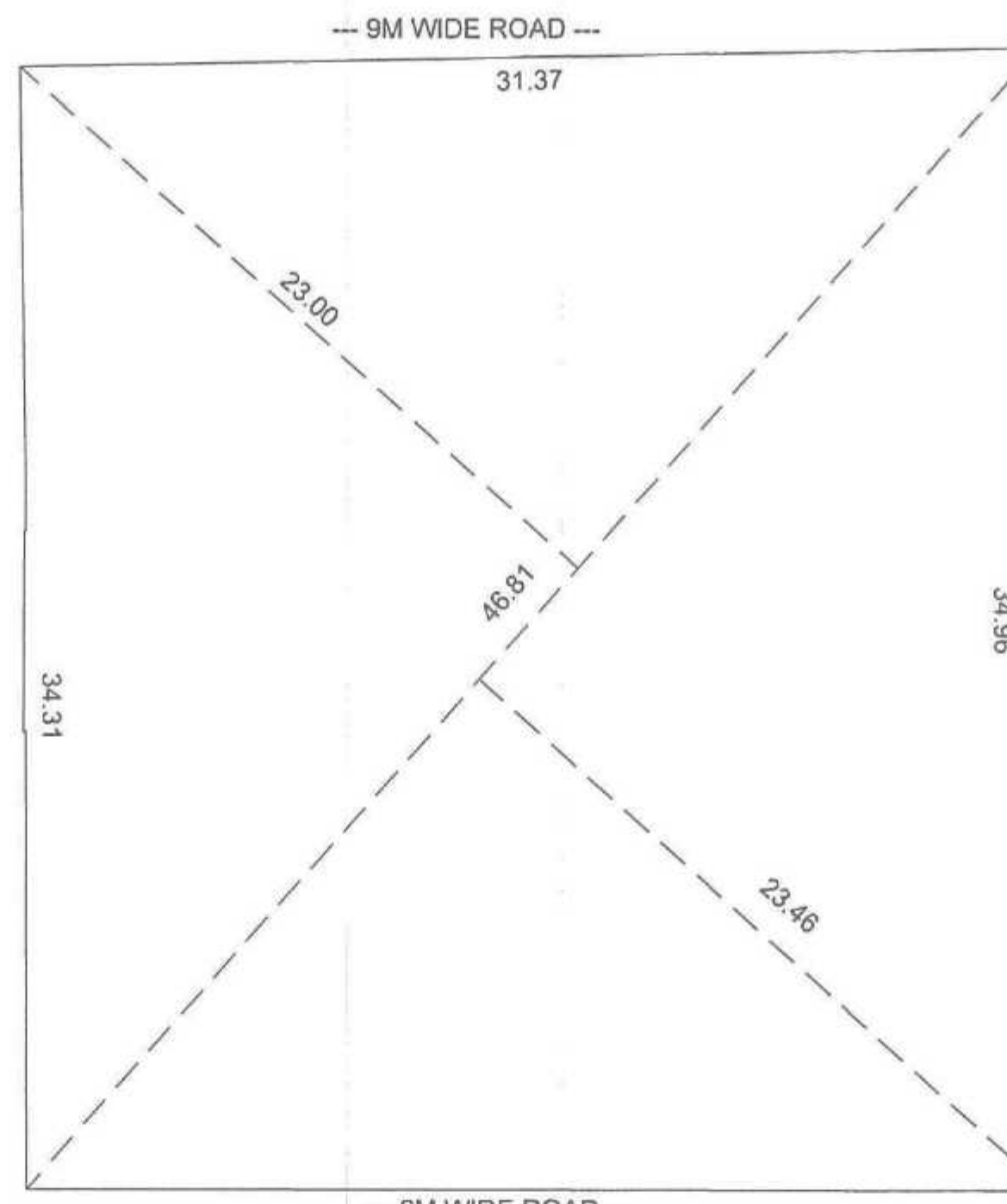
PLOT AREA CALC. BY TRIGULATION METHOD
