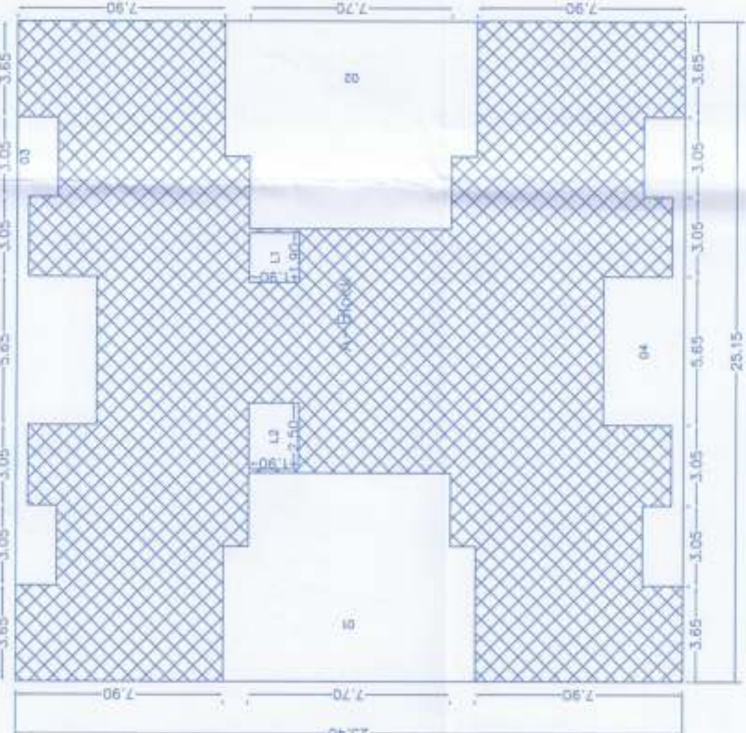
TYPICAL - 7, 9 &amp; 11 FLOOR PLAN
