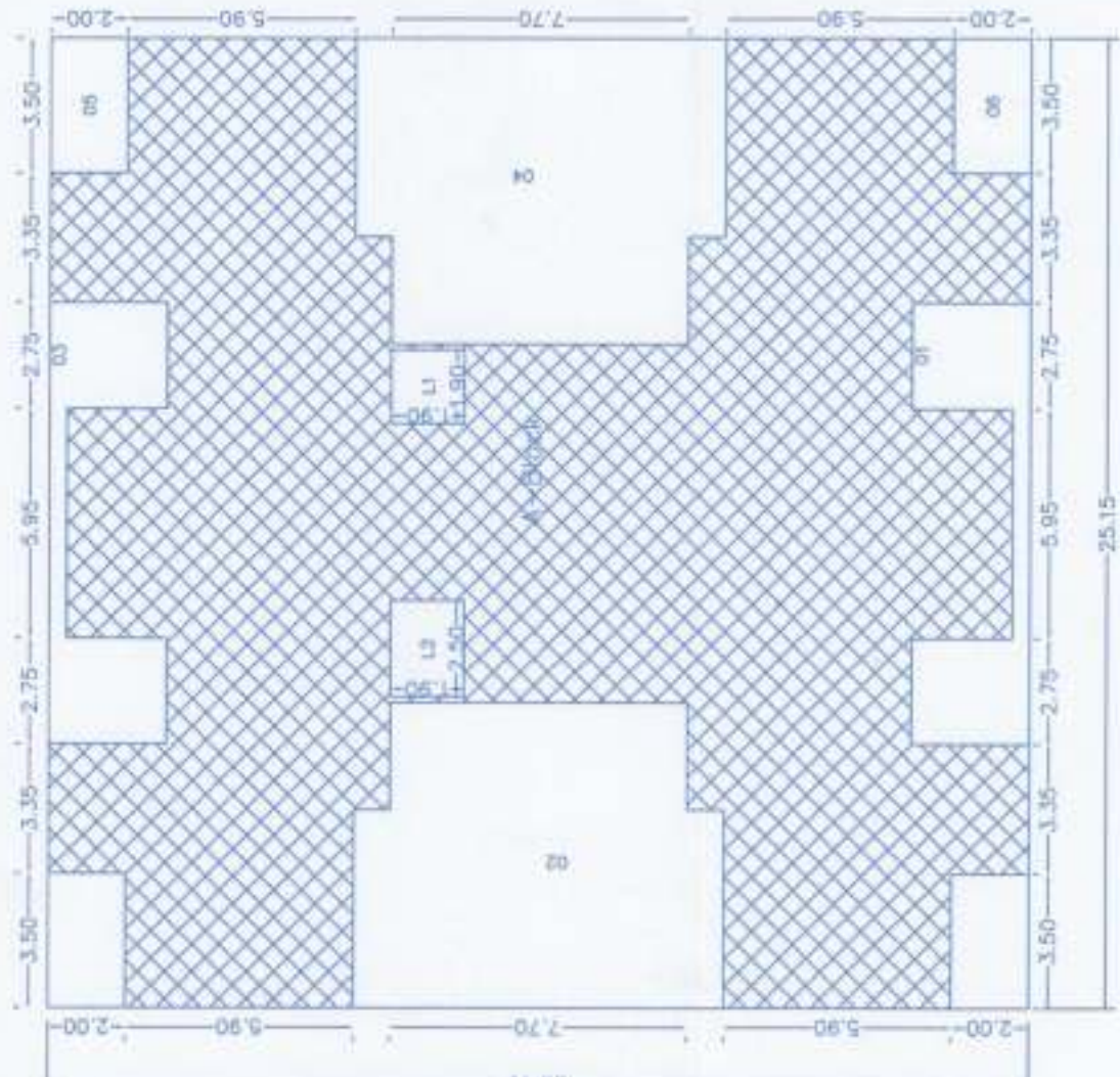
TYPICAL - 10&amp; 12 FLOOR PLAN
