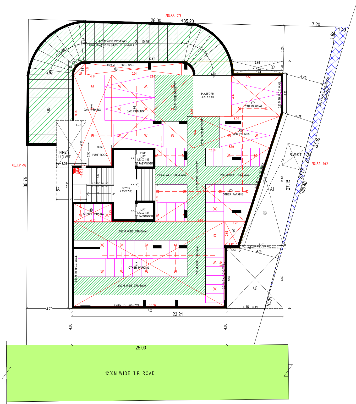
BASEMENT PLAN SCALE:- 1CM. = 1.00 M.
