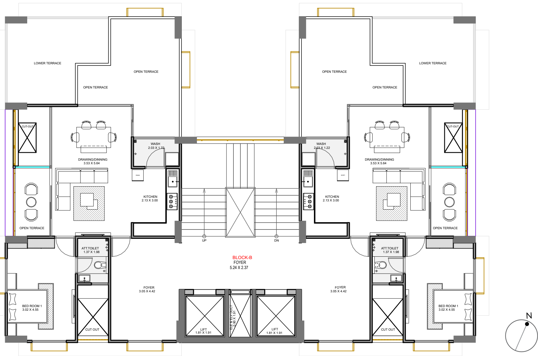
BLOCK B 14 th FLOOR TYPICAL PLAN
