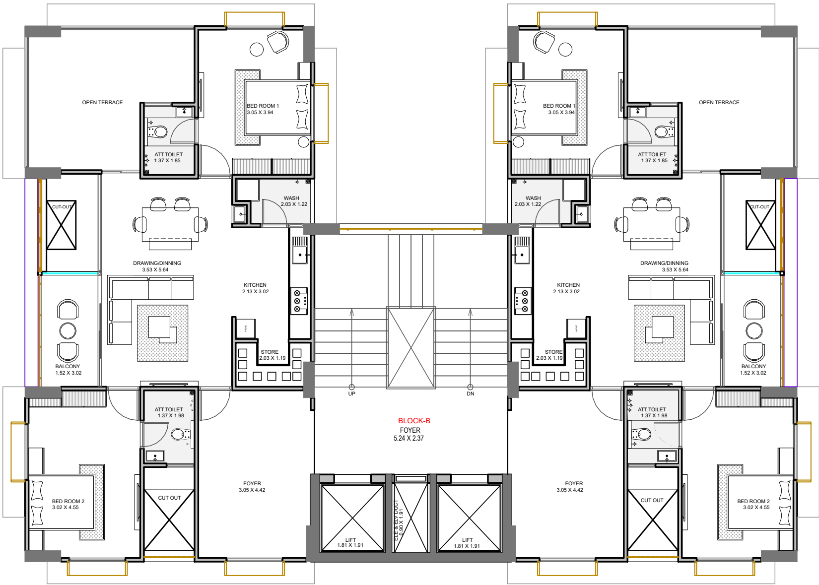
BLOCK B 14 th FLOOR TYPICAL PLAN
