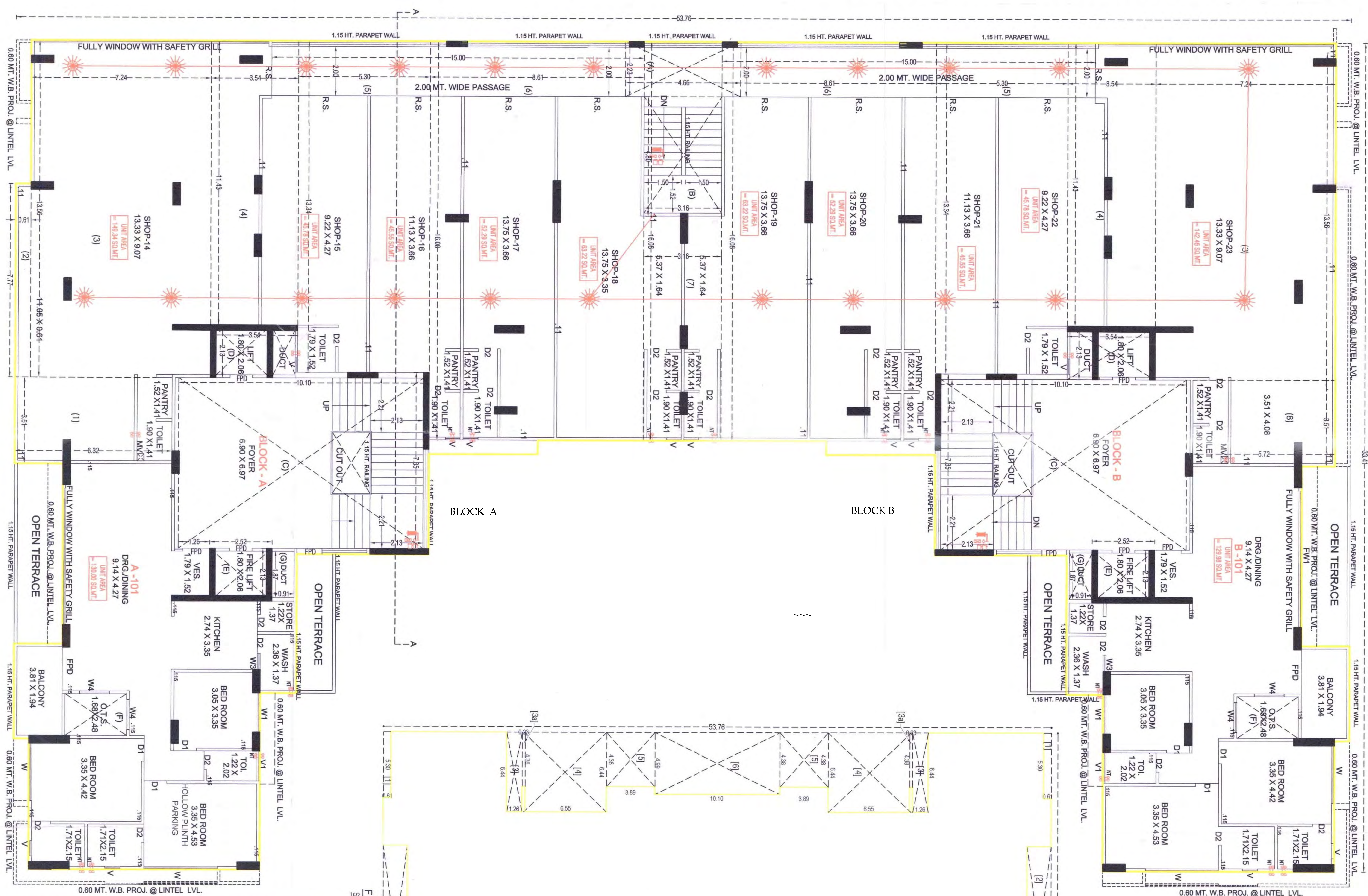
FIRST FLOOR PLAN SCALE :- 1:100 CM. = 2.00 MT.
