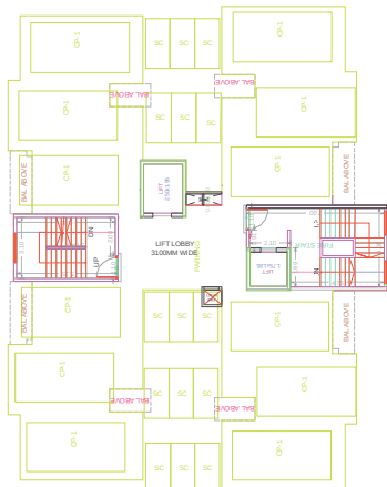
STILT PARKING FLOOR PLAN
