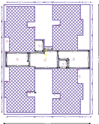
TYPICAL - 1-13 FLOOR PLAN
