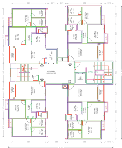
TYPICAL - 1- 13 FLOOR PLAN
