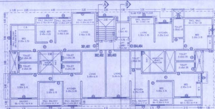
THIRD & FOURTH FLOOR PLAN (RES.) (SCALE - 1:100)
