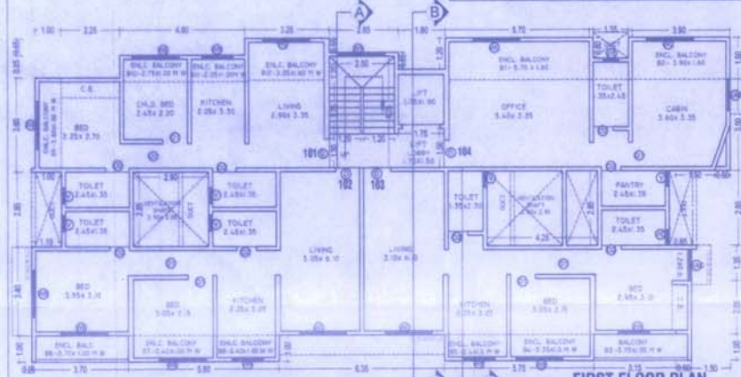
FIRST FLOOR PLAN (RES.) (SCALE - 1:100)
