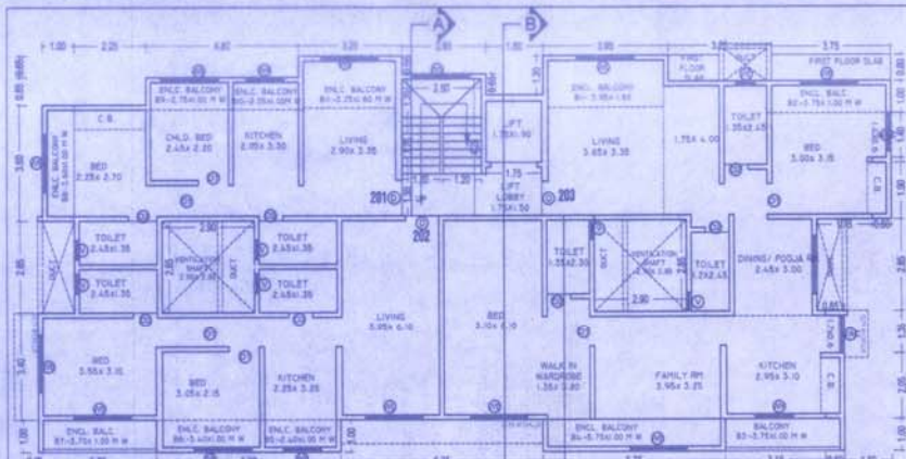
SECOND FLOOR PLAN (RES.) (SCALE - 1:100)
