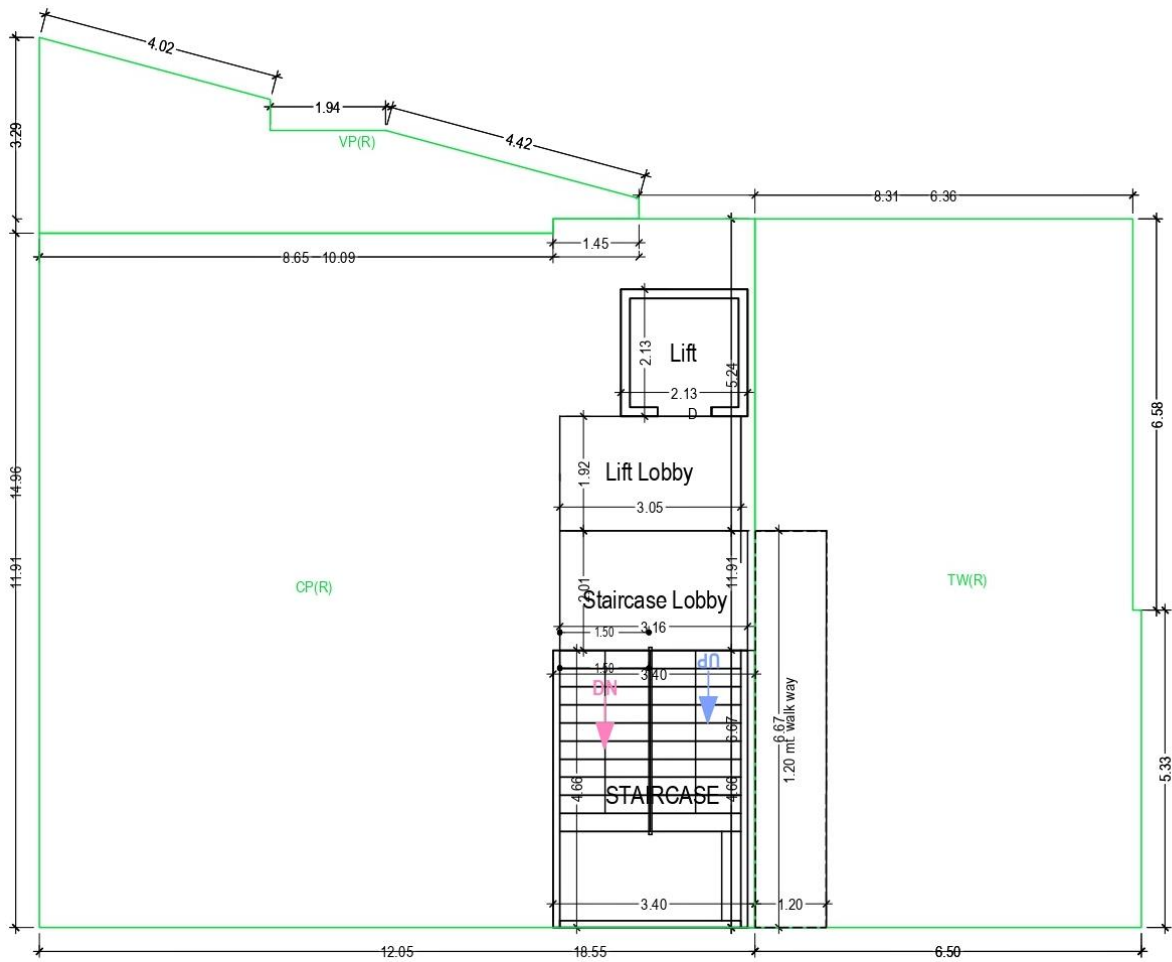
PARKING FLOOR PLAN (SCALE 1:100)
