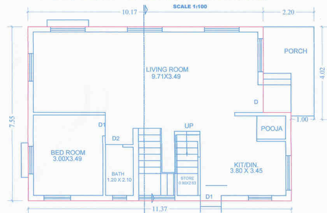
GROUND FLOOR PLAN OF BUNGALOW -1ST,2ND,3RD,4TH&5TH SCALE 1:100
