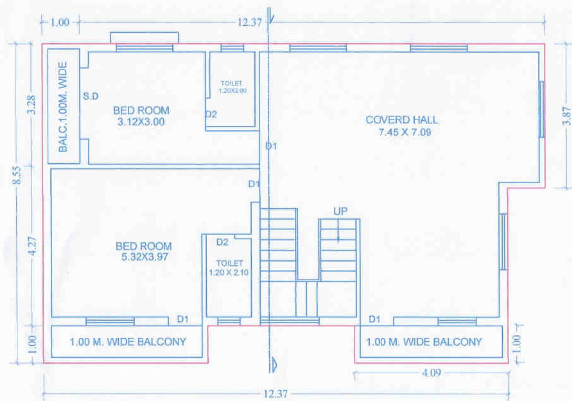
FIRST FLOOR PLAN OF BUNGALOW -1ST,2ND,3RD,4TH&5TH SCALE 1:100
