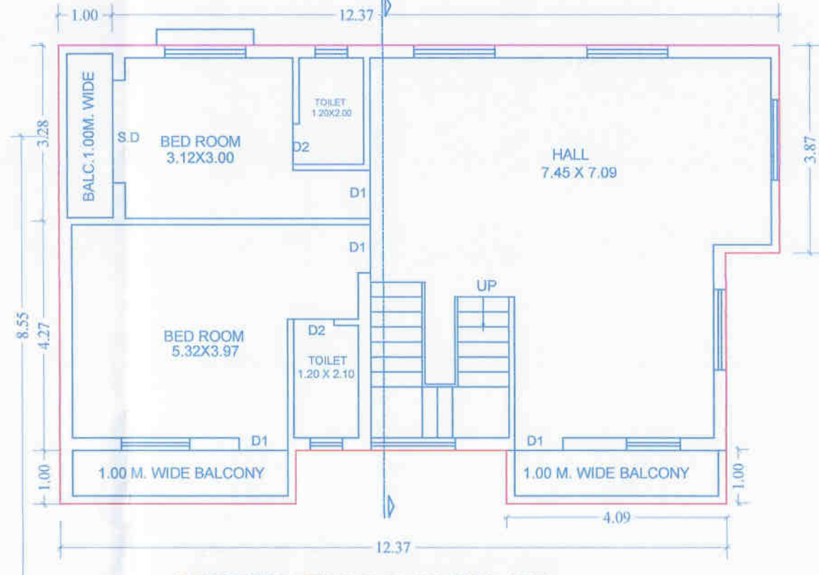
SECOND FLOOR PLAN OF BUNGALOW -1ST,2ND,3RD,4TH&5TH SCALE 1:100
