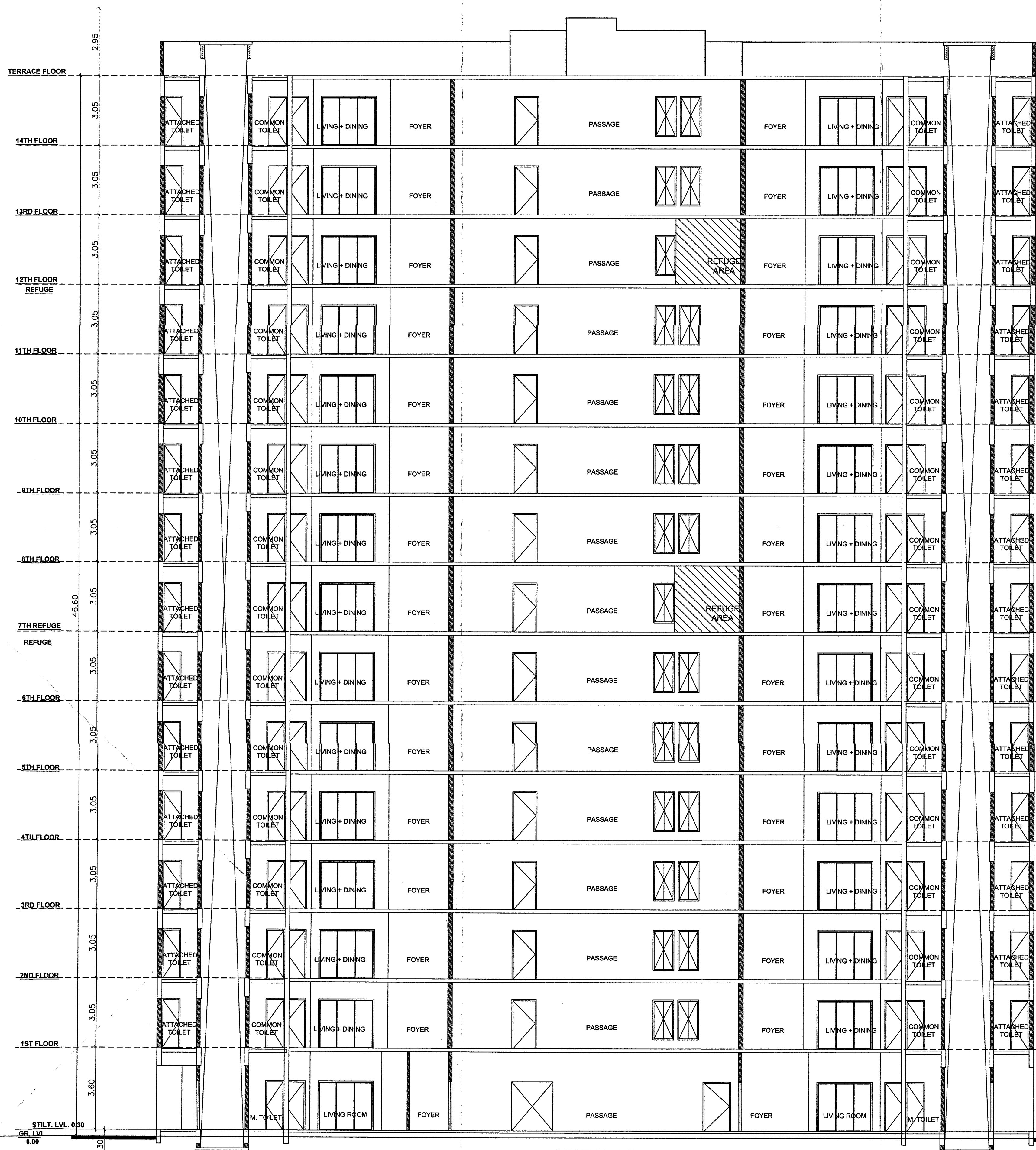
SECTION AA'
