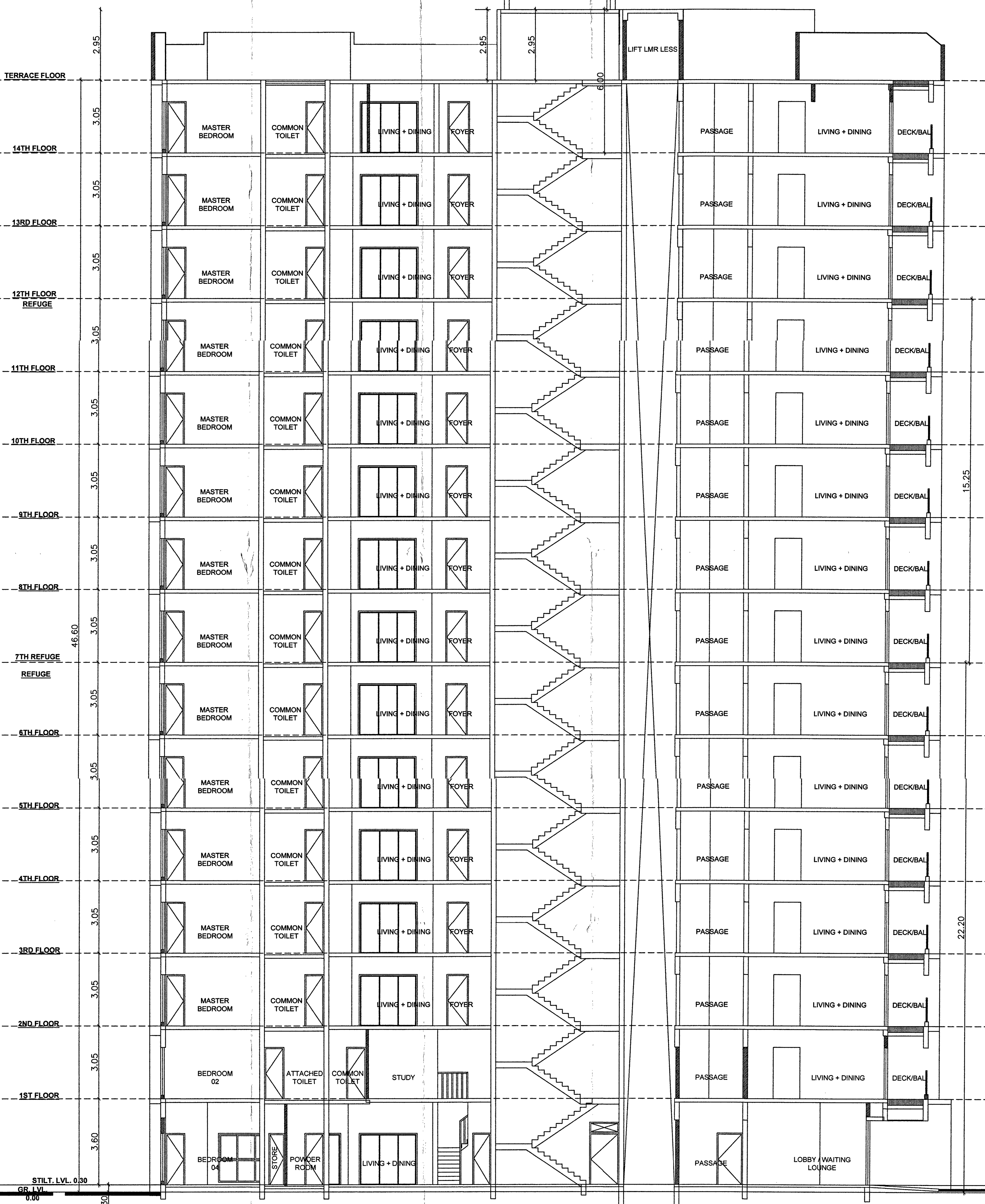
SECTION BB'
