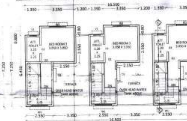
TYPICAL SECOND FLOOR PLAN (BUILDING 'E') SCALE 1:100
