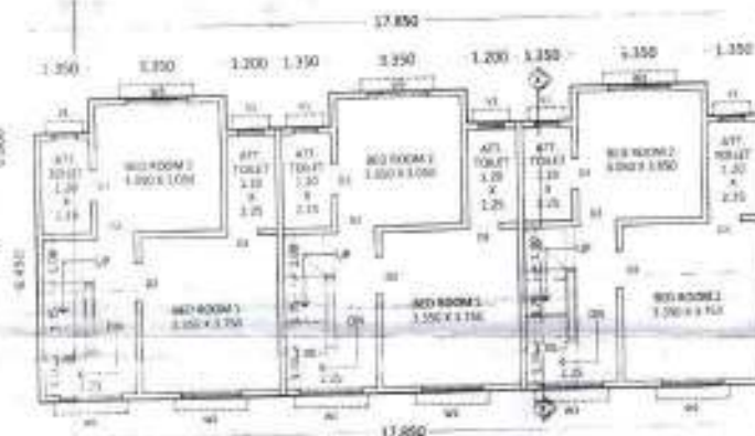
TYPICAL FIRST FLOOR PLAN (BUILDING 'E') SCALE 1:100
