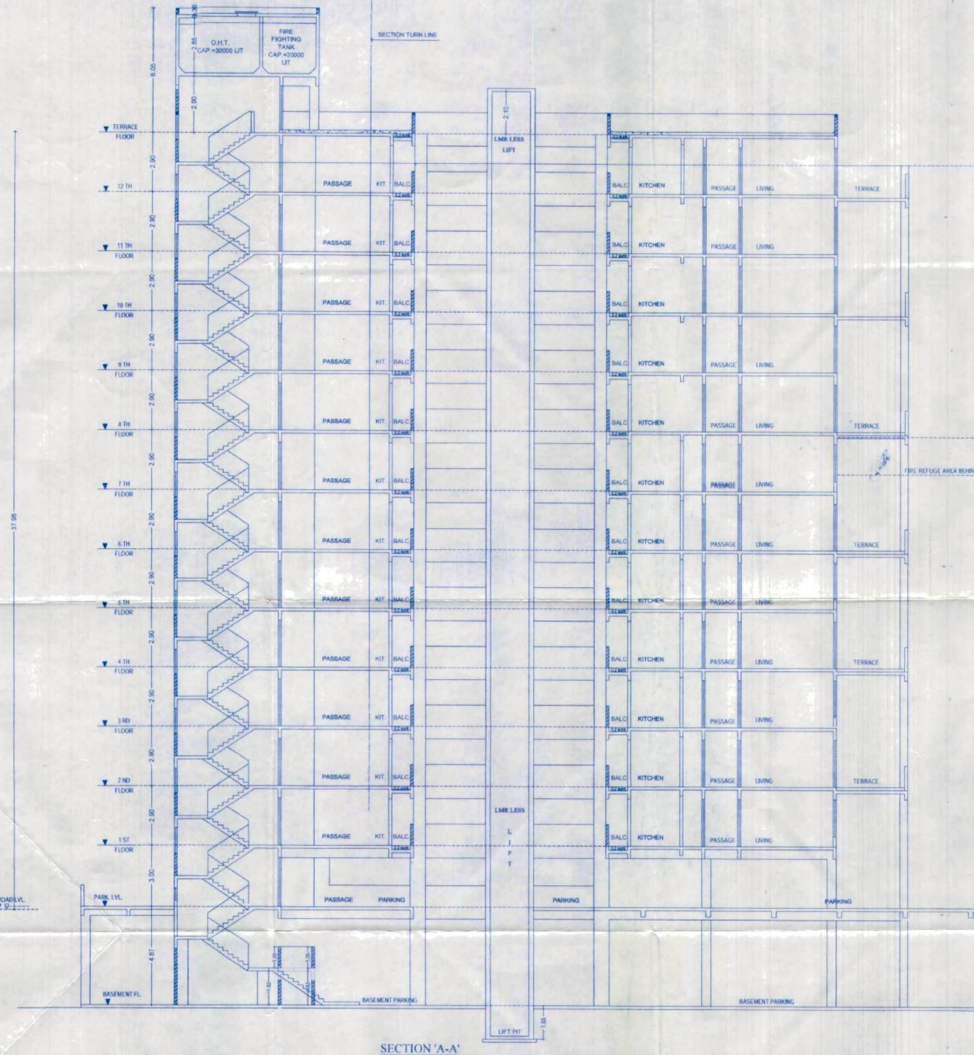
SECTION 'A-A'
