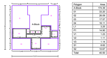
SIXTH FLOOR PLAN
