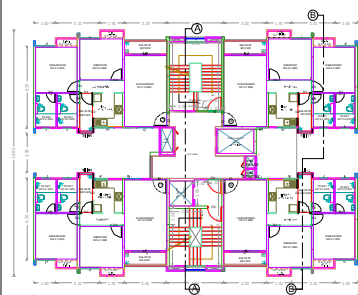
TYPICAL - 1- 19 FLOOR PLAN
