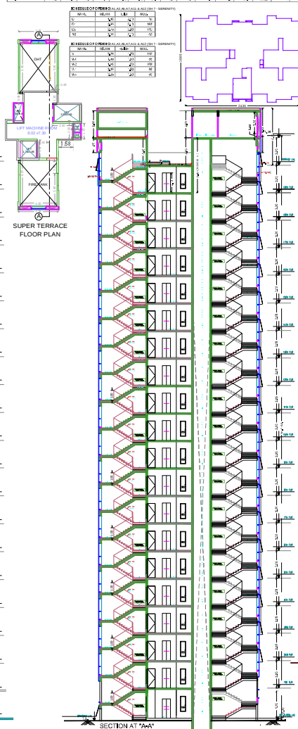
SECTION AT "A-A"
