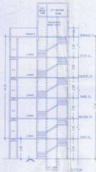
SECTION
