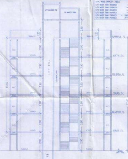
SECTION B-B FIRE STAIR CASE SECTION
