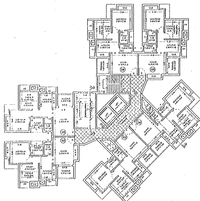
TYPICAL (3RD, 7TH, 9TH, 11TH & 15TH) FLOOR PLAN BLDG-D05 & D08 SCALE: 1:100
