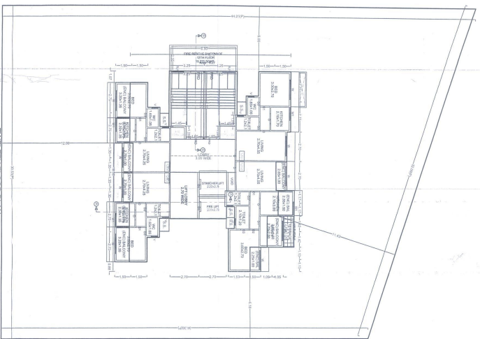
TWELFTH FLOOR PLAN
