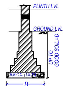
TYP. WALL SECTION FOR 0.23 THK. WALL
