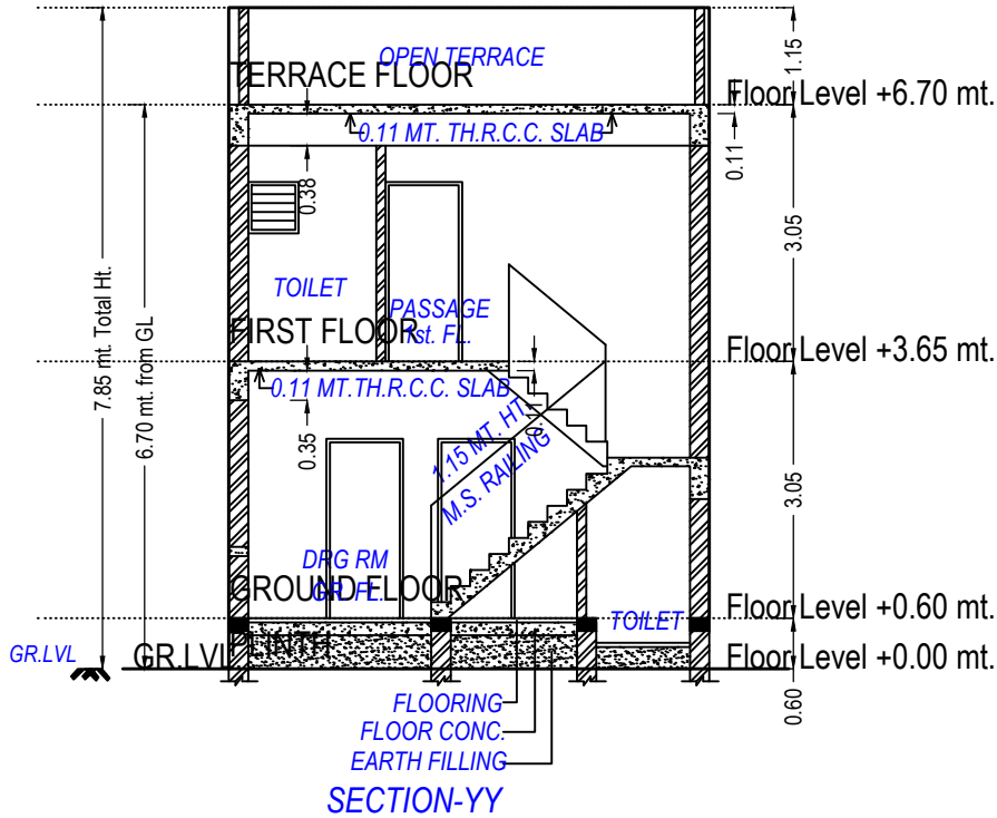
SECTION-YY
