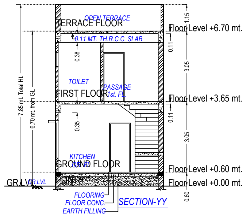
SECTION-YY
