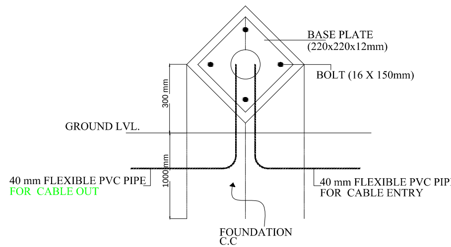
DETAIL AT-A
