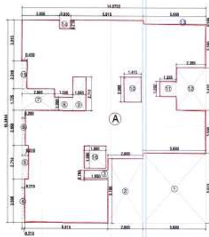
AREA DIAGRAM OF TYPICAL 1ST TO 3RD FLOORS
