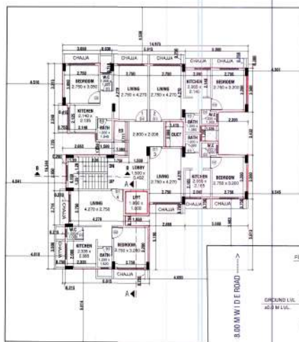
TYPICAL 1ST TO 3RD FLOOR PLAN
