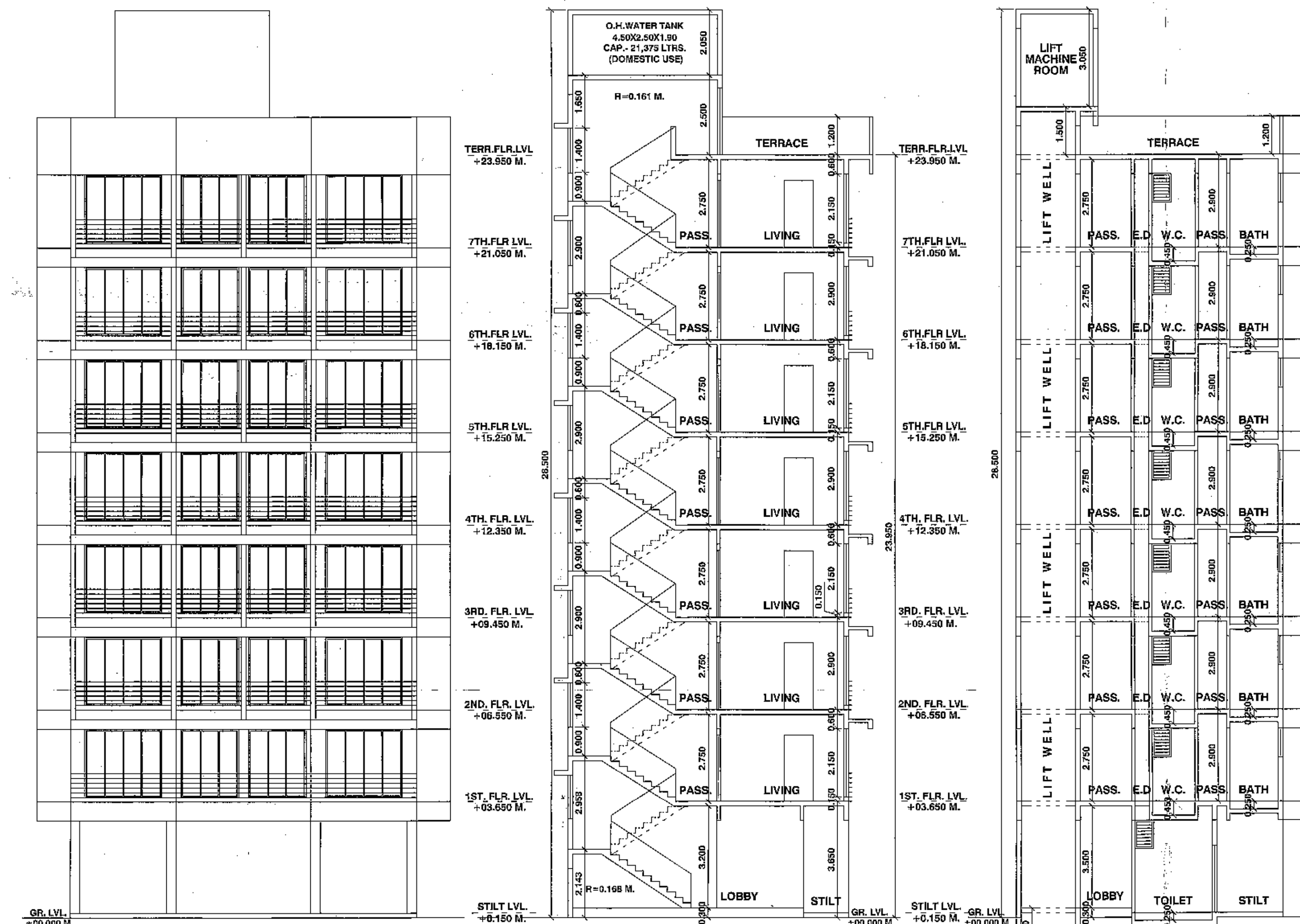
FRONT SIDE ELEVATION SCALE = 1:100
