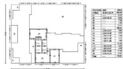
TYPICAL - 4, 6, 8, 10, 12, 14 & 16 FLOOR PLAN
