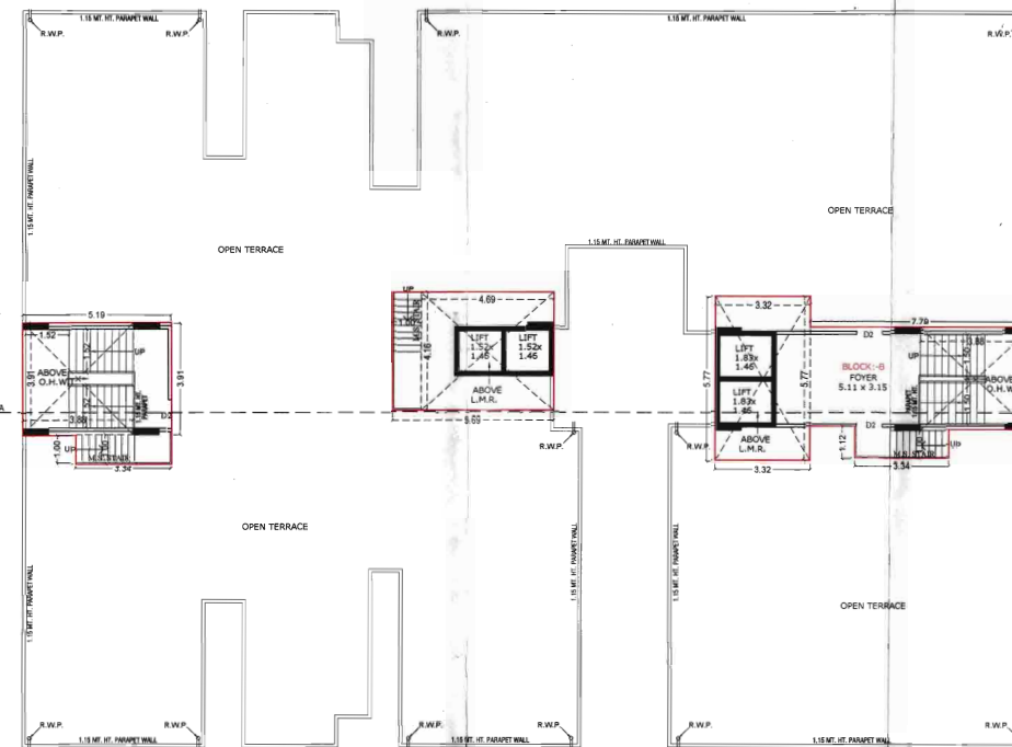
STAIR CABIN, LIFT MACHINE RM, O.H.W.T. & OPEN TERRACE PLAN
