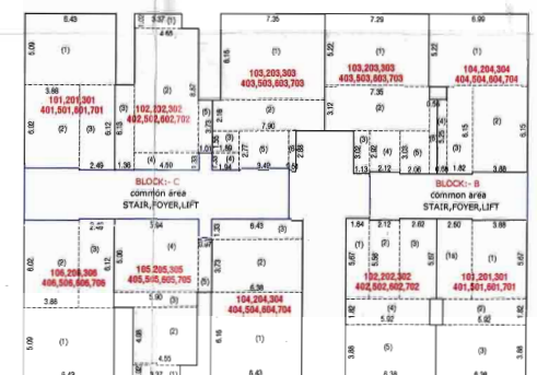
1st to 7th FL. (UNIT BUILT UP AREA CAL.)
