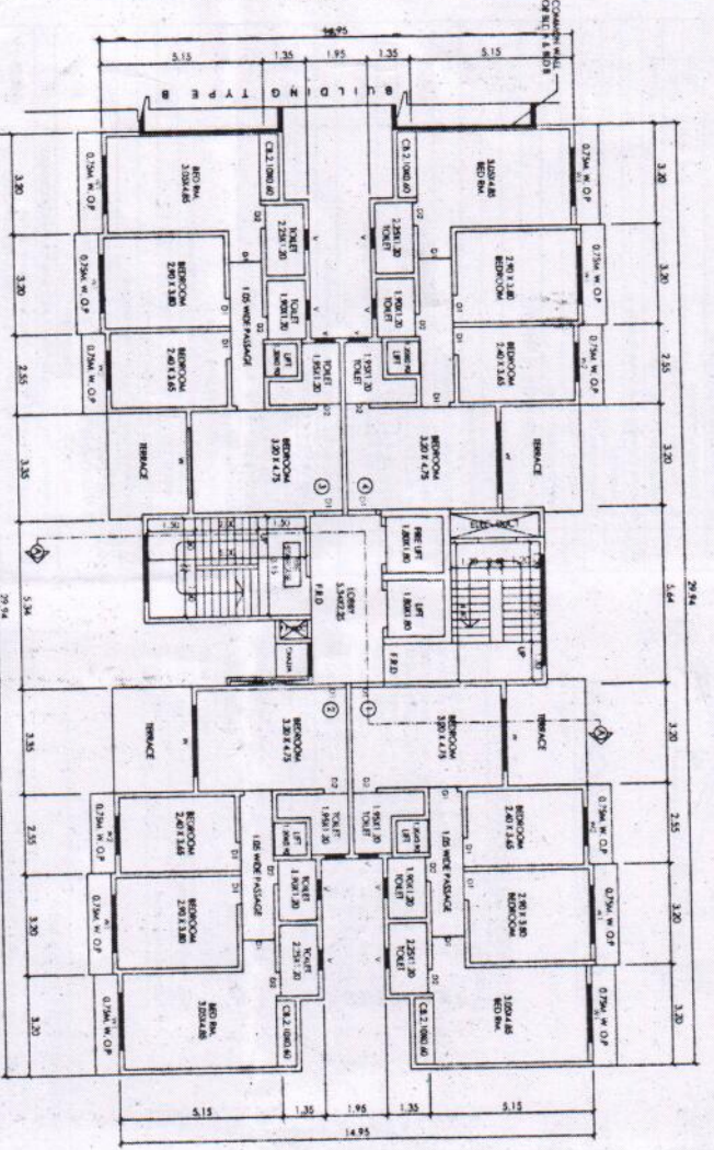
24TH FLOOR PLAN
