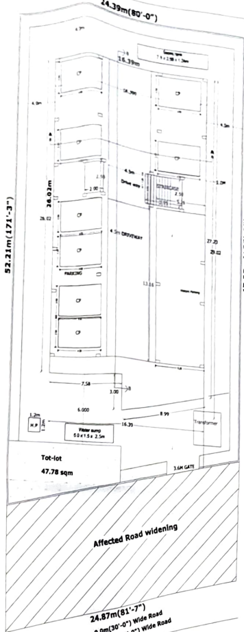
STILT FLOOR PLAN (SCALE 1:100)
