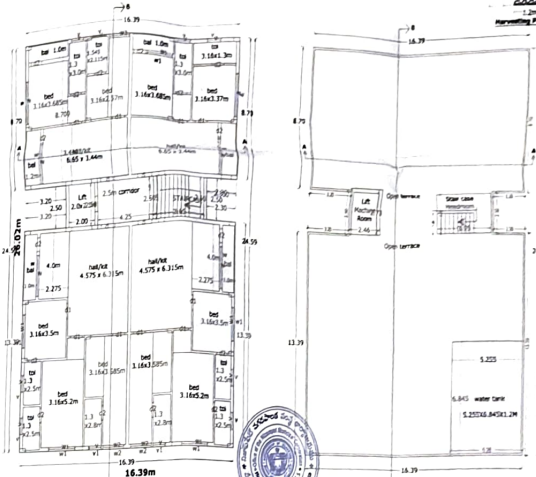
SECOND, THIRD, FOURTH & FIFTH FLOOR PLAN (SCALE 1:100)
