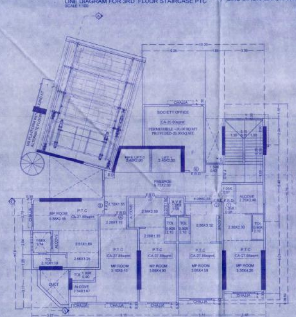
3RD FLOOR PLAN (PTC) WING A SCALE 1:100
