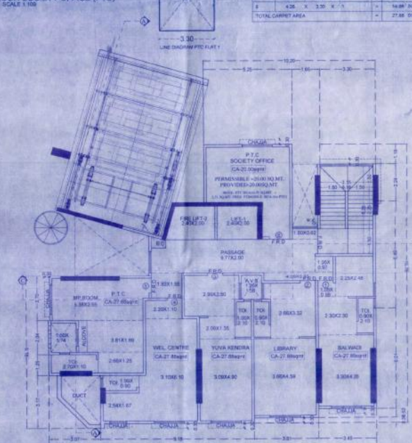
4TH FLOOR PLAN (PTC) WING A SCALE 1:100
