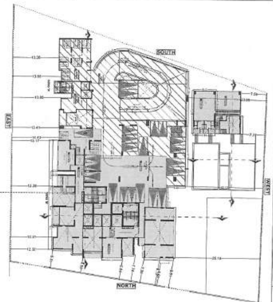
WING-B METER ROOM SCALE - 1:100
